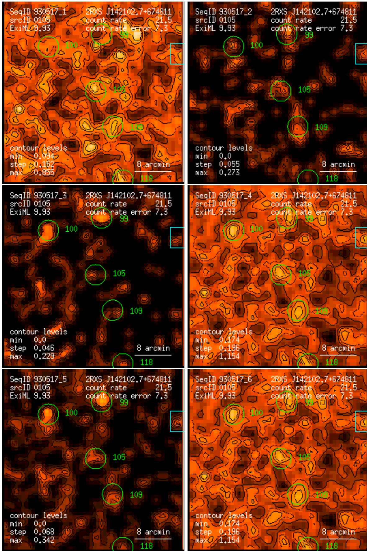
Figure 105: RASS 930517: detection 0105: band rate images, Gaussian filter: (1) PSPC channels 11 – 41, (2) 52 – 90, (3) 91 – 201, (4) 11 – 235, (5) 52 – 201, (6) 11 – 201. Broad band rates in counts/ks. Band rate contour levels in counts/ks/arcmin 2 .
