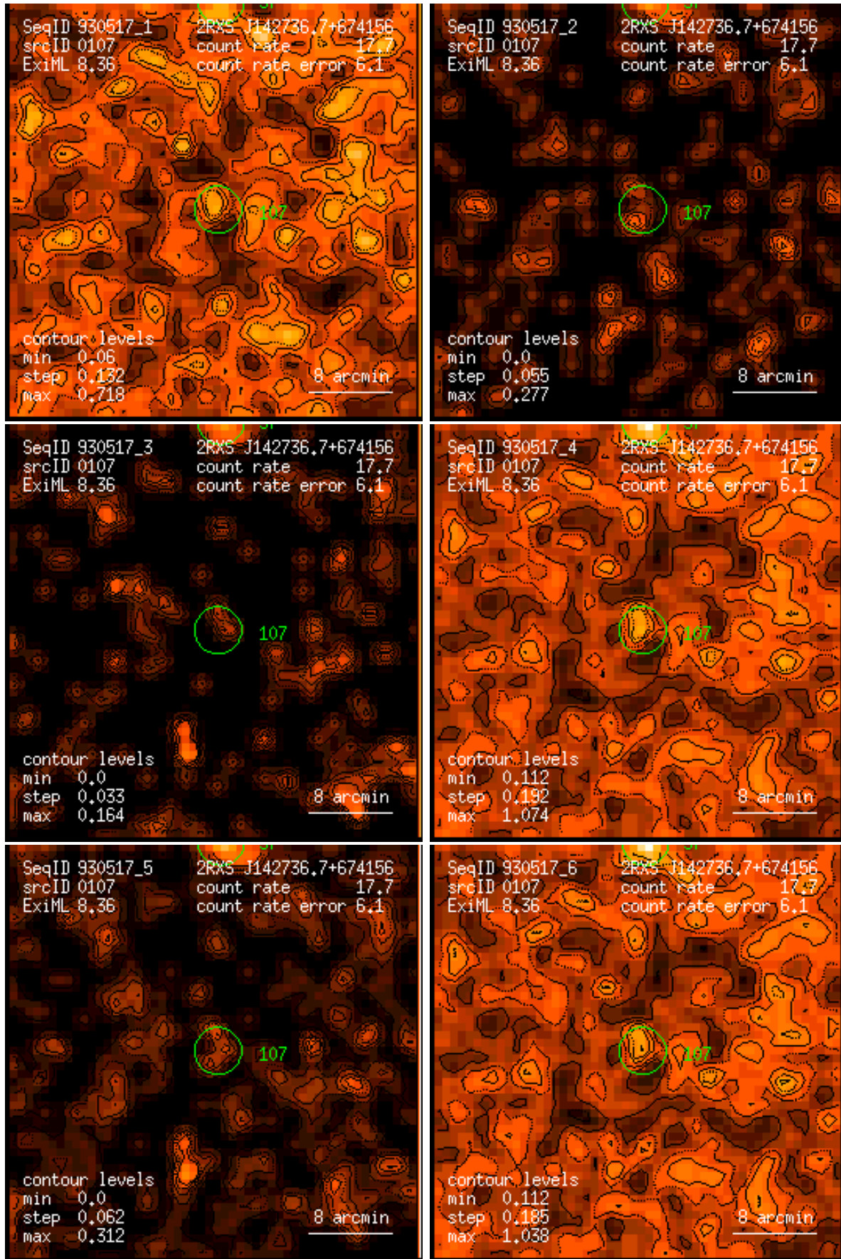
Figure 107: RASS 930517: detection 0107: band rate images, Gaussian filter: (1) PSPC channels 11 – 41, (2) 52 – 90, (3) 91 – 201, (4) 11 – 235, (5) 52 – 201, (6) 11 – 201. Broad band rates in counts/ks. Band rate contour levels in counts/ks/arcmin 2 .
