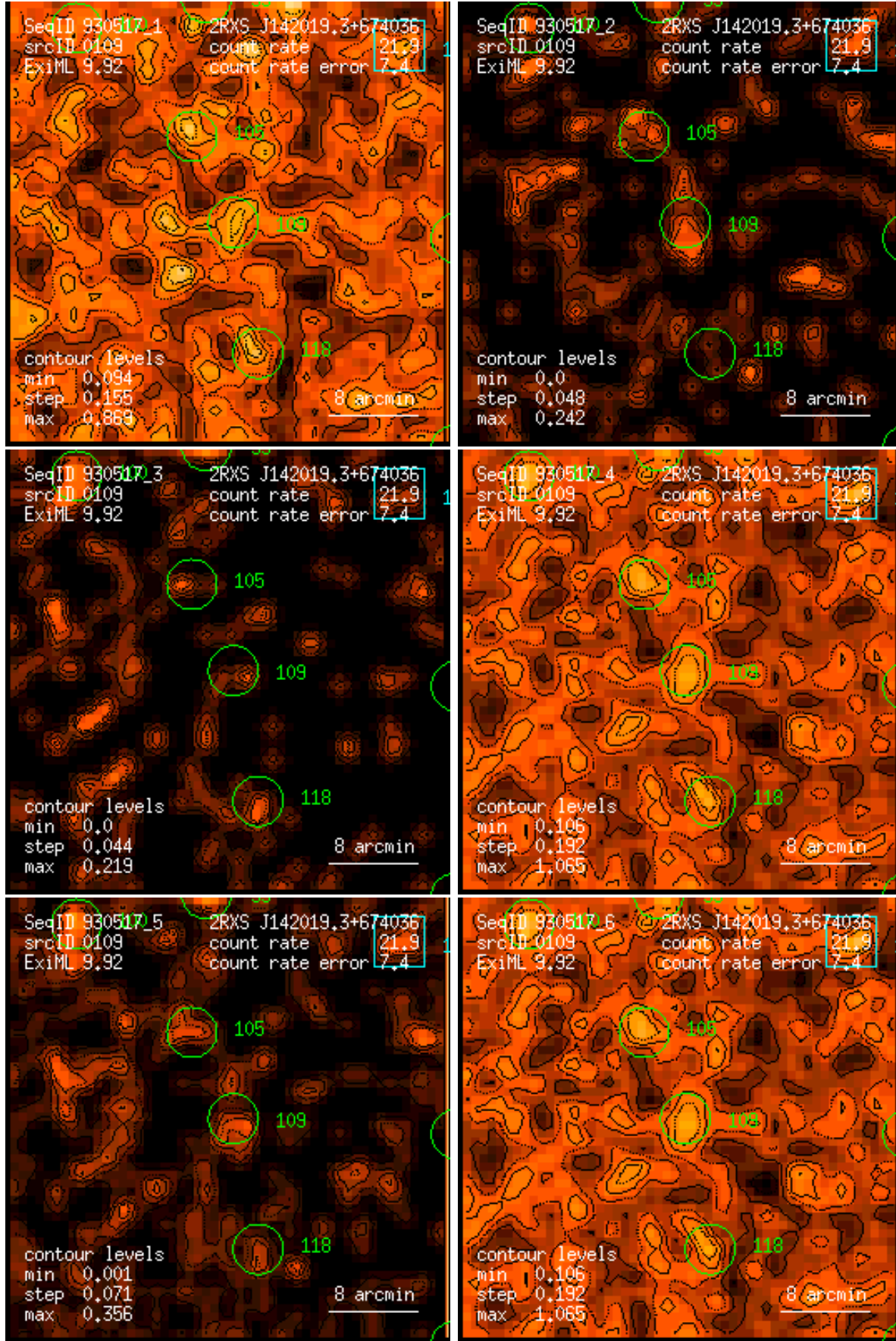
Figure 109: RASS 930517: detection 0109: band rate images, Gaussian filter: (1) PSPC channels 11 – 41, (2) 52 – 90, (3) 91 – 201, (4) 11 – 235, (5) 52 – 201, (6) 11 – 201. Broad band rates in counts/ks. Band rate contour levels in counts/ks/arcmin 2 .
