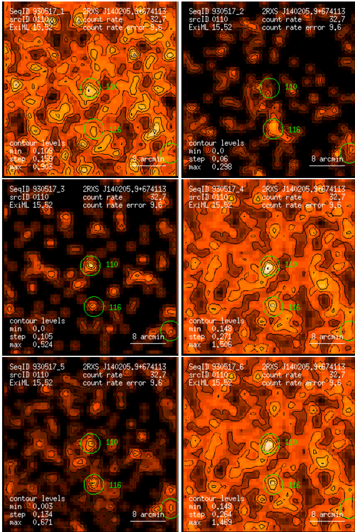
Figure 110: RASS 930517: detection 0110: band rate images, Gaussian filter: (1) PSPC channels 11 – 41, (2) 52 – 90, (3) 91 – 201, (4) 11 – 235, (5) 52 – 201, (6) 11 – 201. Broad band rates in counts/ks. Band rate contour levels in counts/ks/arcmin 2 .
