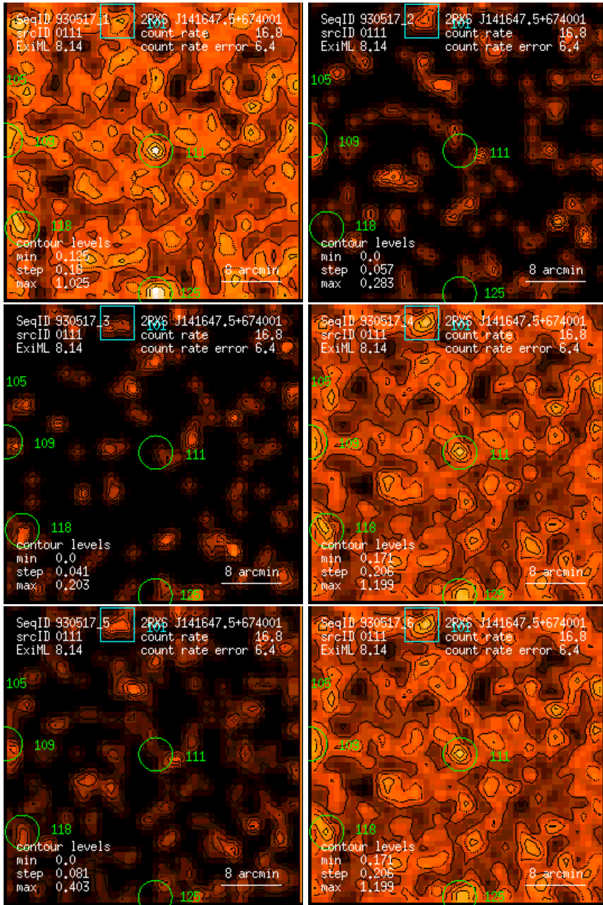
Figure 111: RASS 930517: detection 0111: band rate images, Gaussian filter: (1) PSPC channels 11 – 41, (2) 52 – 90, (3) 91 – 201, (4) 11 – 235, (5) 52 – 201, (6) 11 – 201. Broad band rates in counts/ks. Band rate contour levels in counts/ks/arcmin 2 .
