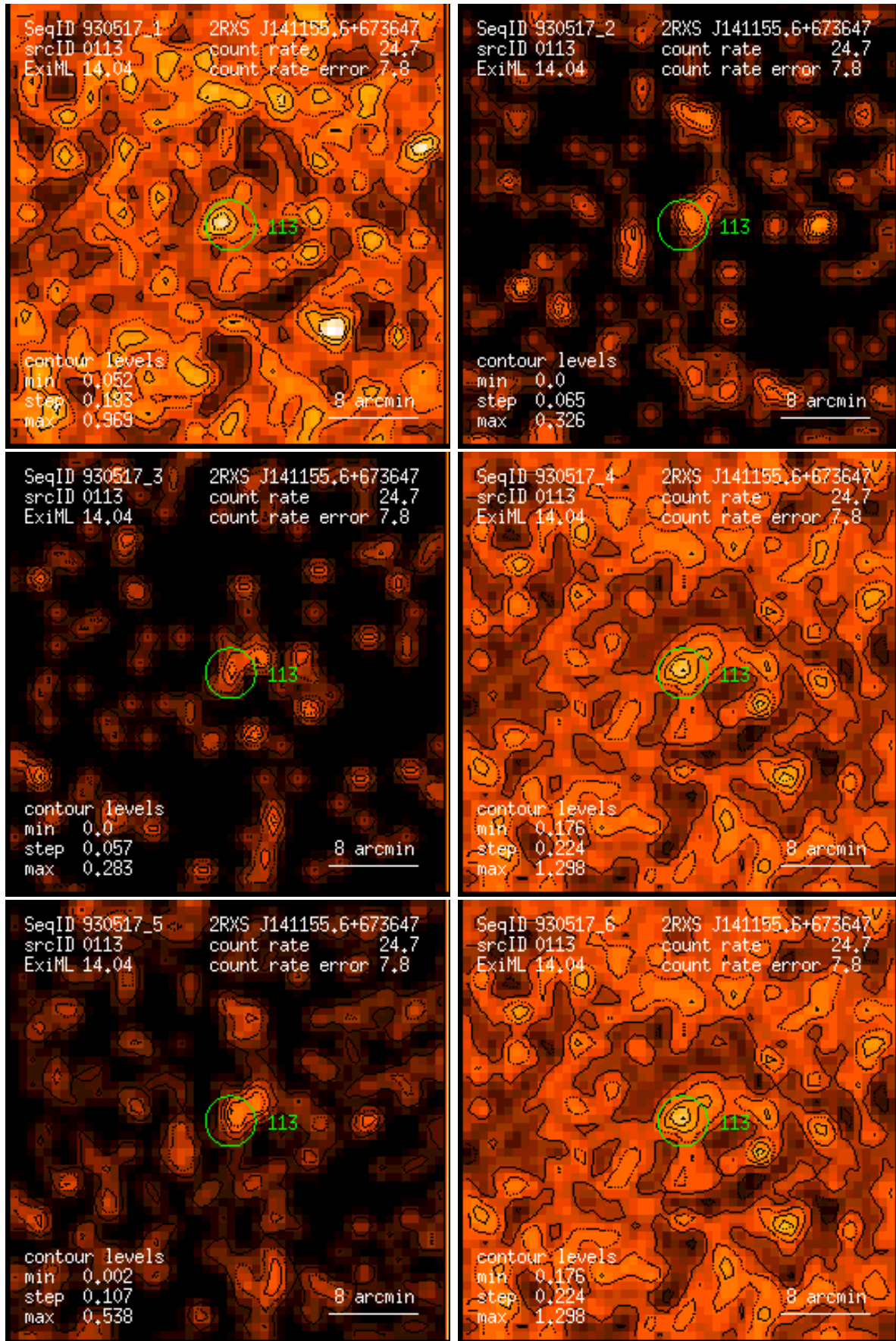
Figure 113: RASS 930517: detection 0113: band rate images, Gaussian filter: (1) PSPC channels 11 – 41, (2) 52 – 90, (3) 91 – 201, (4) 11 – 235, (5) 52 – 201, (6) 11 – 201. Broad band rates in counts/ks. Band rate contour levels in counts/ks/arcmin 2 .
