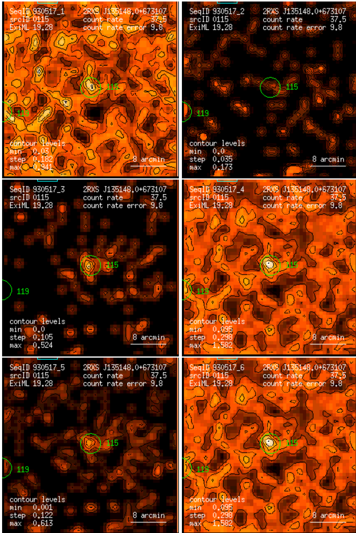
Figure 115: RASS 930517: detection 0115: band rate images, Gaussian filter: (1) PSPC channels 11 – 41, (2) 52 – 90, (3) 91 – 201, (4) 11 – 235, (5) 52 – 201, (6) 11 – 201. Broad band rates in counts/ks. Band rate contour levels in counts/ks/arcmin 2 .
