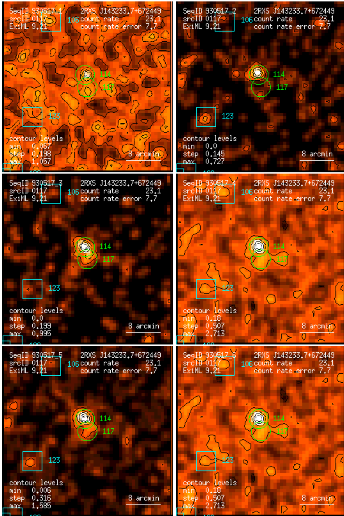
Figure 117: RASS 930517: detection 0117: band rate images, Gaussian filter: (1) PSPC channels 11 – 41, (2) 52 – 90, (3) 91 – 201, (4) 11 – 235, (5) 52 – 201, (6) 11 – 201. Broad band rates in counts/ks. Band rate contour levels in counts/ks/arcmin 2 .
