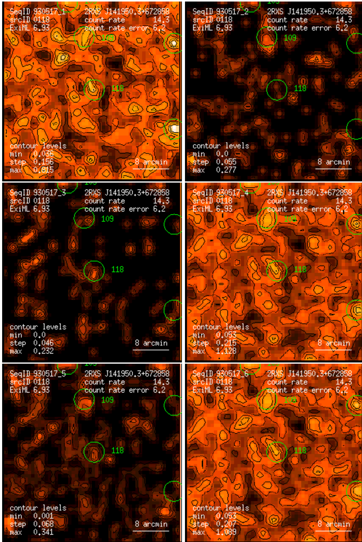
Figure 118: RASS 930517: detection 0118: band rate images, Gaussian filter: (1) PSPC channels 11 – 41, (2) 52 – 90, (3) 91 – 201, (4) 11 – 235, (5) 52 – 201, (6) 11 – 201. Broad band rates in counts/ks. Band rate contour levels in counts/ks/arcmin 2 .
