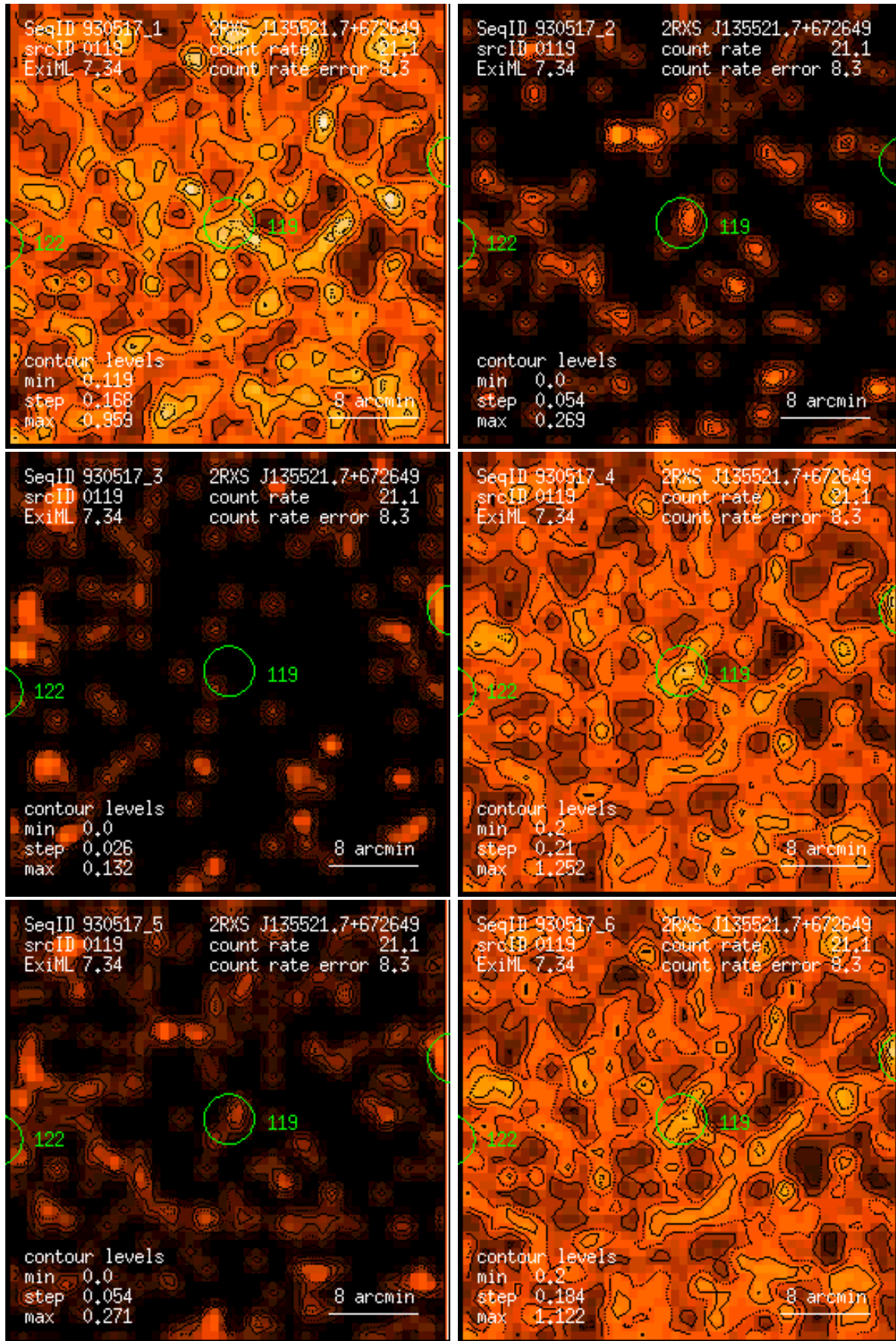
Figure 119: RASS 930517: detection 0119: band rate images, Gaussian filter: (1) PSPC channels 11 – 41, (2) 52 – 90, (3) 91 – 201, (4) 11 – 235, (5) 52 – 201, (6) 11 – 201. Broad band rates in counts/ks. Band rate contour levels in counts/ks/arcmin 2 .
