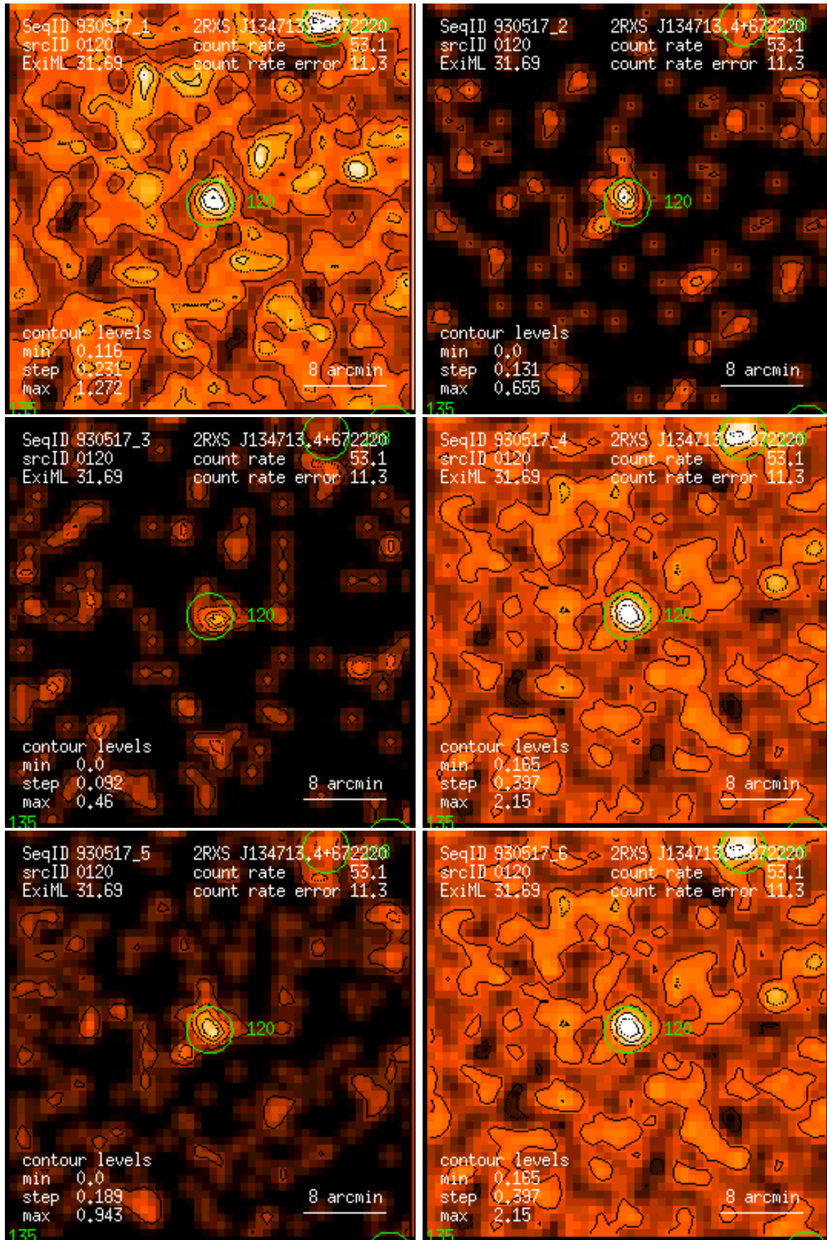
Figure 120: RASS 930517: detection 0120: band rate images, Gaussian filter: (1) PSPC channels 11 – 41, (2) 52 – 90, (3) 91 – 201, (4) 11 – 235, (5) 52 – 201, (6) 11 – 201. Broad band rates in counts/ks. Band rate contour levels in counts/ks/arcmin 2 .
