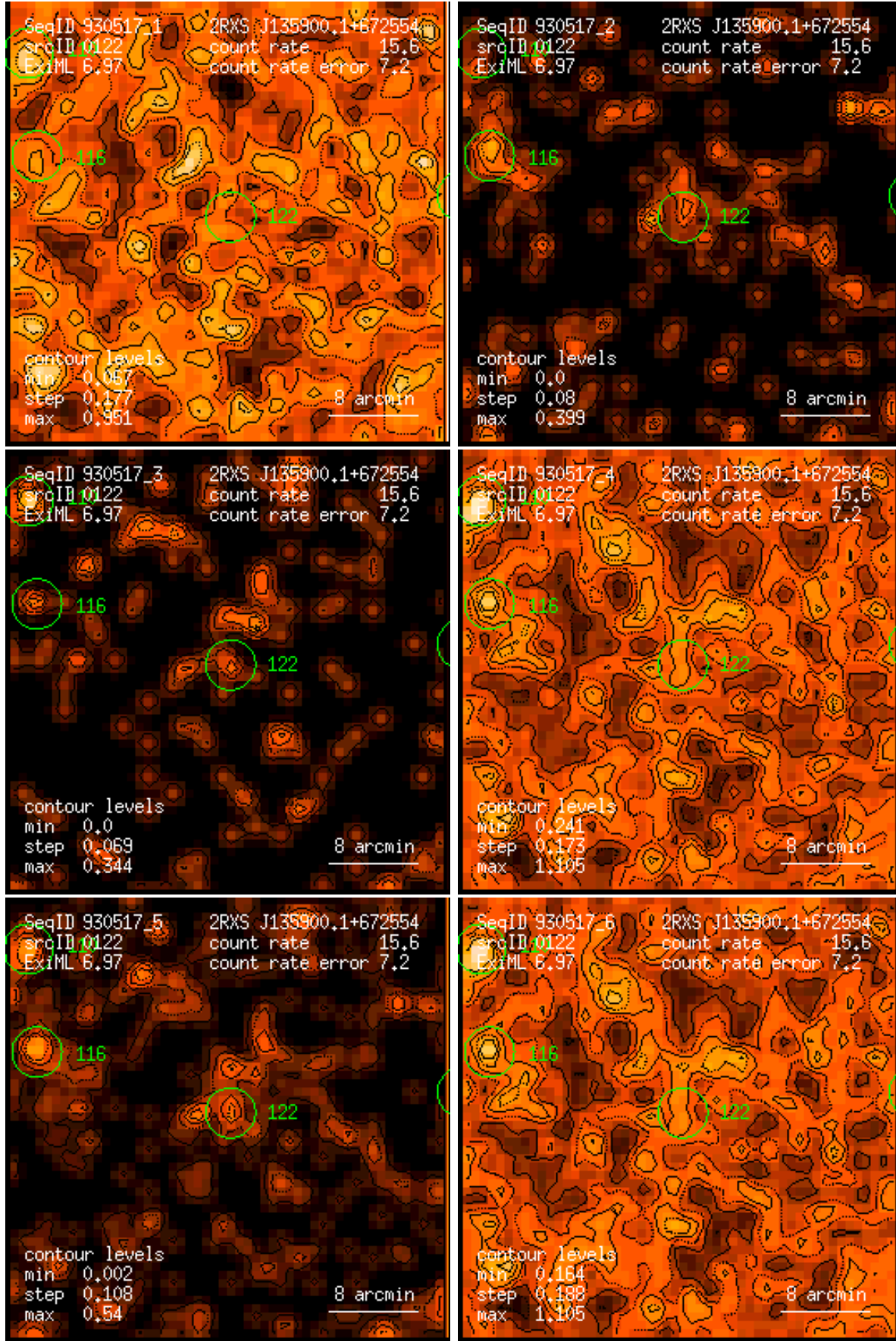
Figure 122: RASS 930517: detection 0122: band rate images, Gaussian filter: (1) PSPC channels 11 – 41, (2) 52 – 90, (3) 91 – 201, (4) 11 – 235, (5) 52 – 201, (6) 11 – 201. Broad band rates in counts/ks. Band rate contour levels in counts/ks/arcmin 2 .
