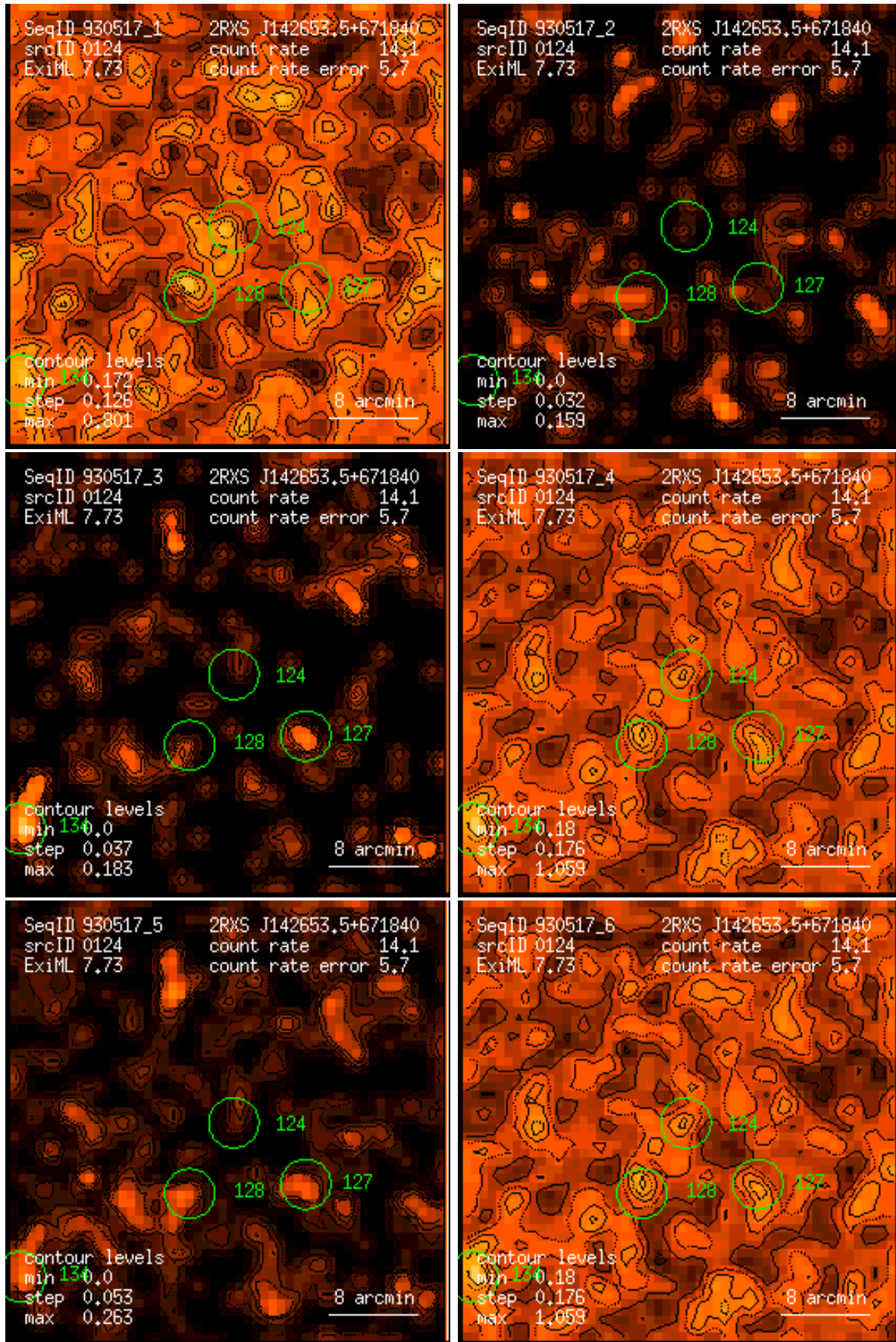
Figure 124: RASS 930517: detection 0124: band rate images, Gaussian filter: (1) PSPC channels 11 – 41, (2) 52 – 90, (3) 91 – 201, (4) 11 – 235, (5) 52 – 201, (6) 11 – 201. Broad band rates in counts/ks. Band rate contour levels in counts/ks/arcmin 2 .
