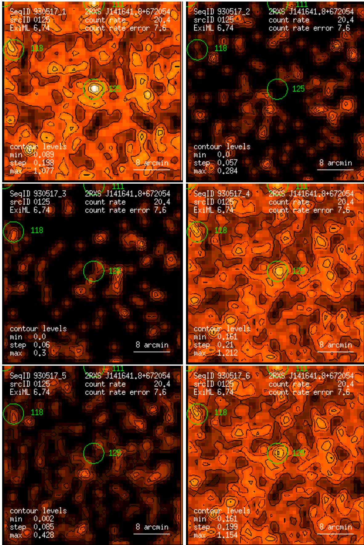
Figure 125: RASS 930517: detection 0125: band rate images, Gaussian filter: (1) PSPC channels 11 – 41, (2) 52 – 90, (3) 91 – 201, (4) 11 – 235, (5) 52 – 201, (6) 11 – 201. Broad band rates in counts/ks. Band rate contour levels in counts/ks/arcmin 2 .
