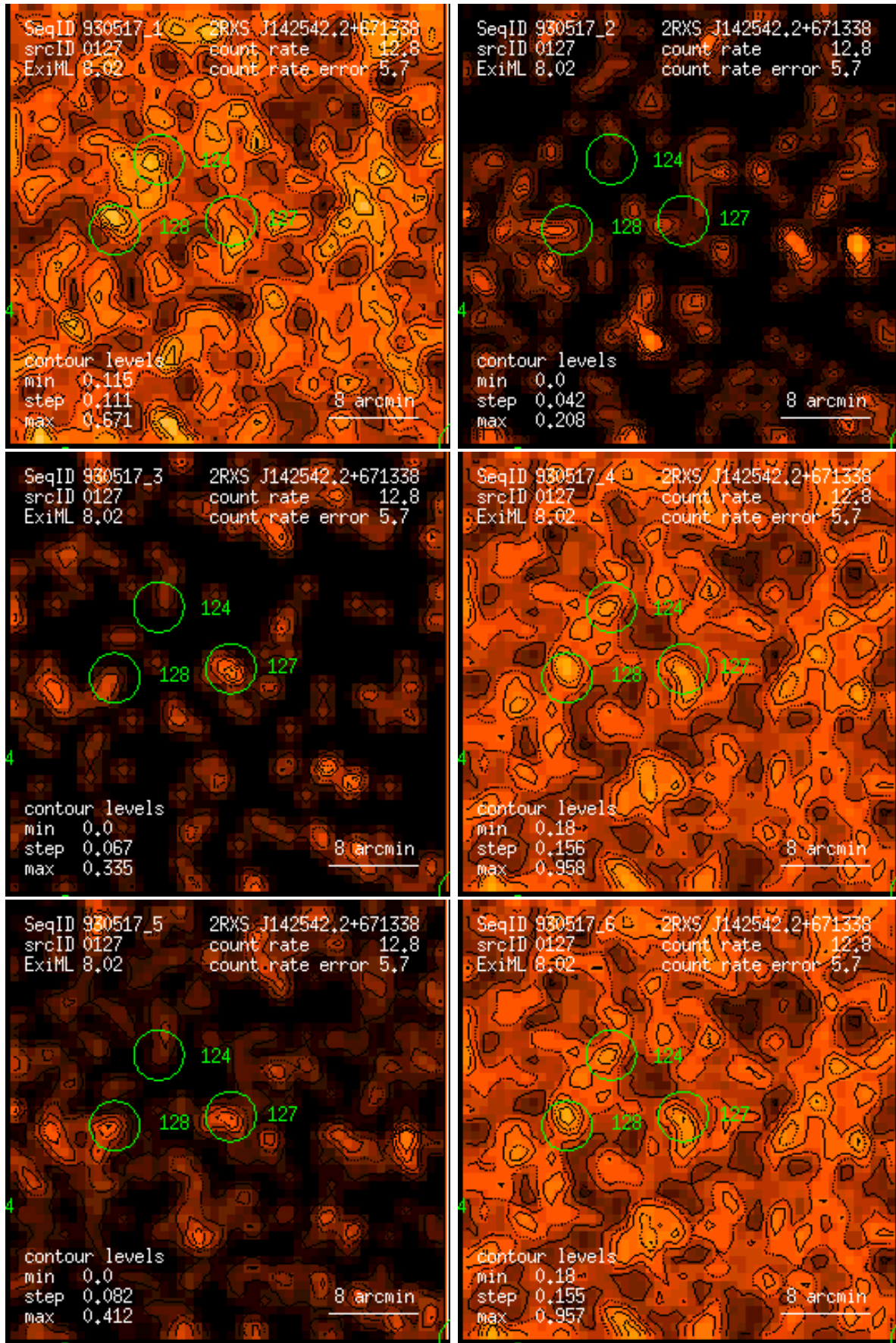
Figure 127: RASS 930517: detection 0127: band rate images, Gaussian filter: (1) PSPC channels 11 – 41, (2) 52 – 90, (3) 91 – 201, (4) 11 – 235, (5) 52 – 201, (6) 11 – 201. Broad band rates in counts/ks. Band rate contour levels in counts/ks/arcmin 2 .
