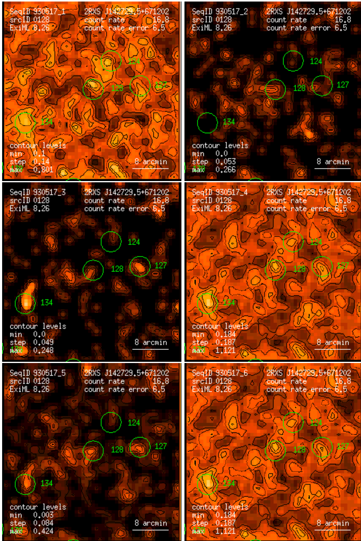
Figure 128: RASS 930517: detection 0128: band rate images, Gaussian filter: (1) PSPC channels 11 – 41, (2) 52 – 90, (3) 91 – 201, (4) 11 – 235, (5) 52 – 201, (6) 11 – 201. Broad band rates in counts/ks. Band rate contour levels in counts/ks/arcmin 2 .
