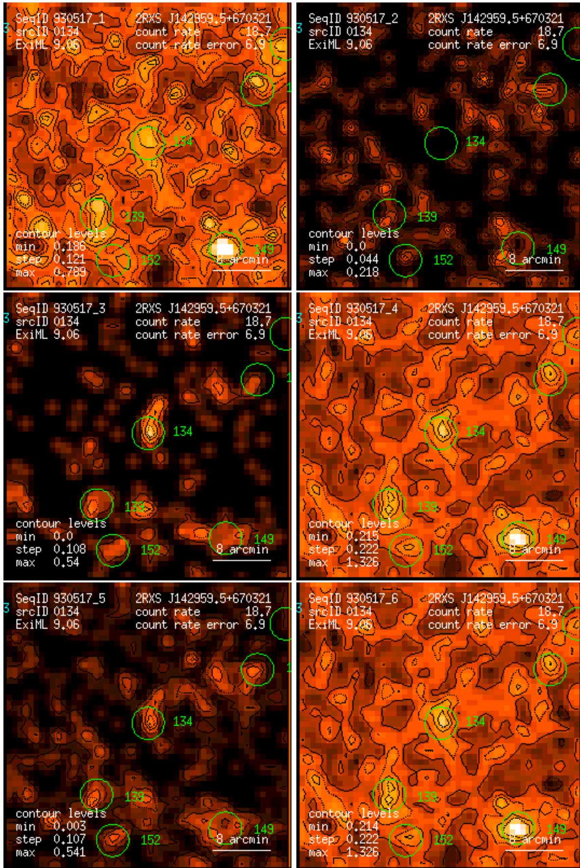
Figure 134: RASS 930517: detection 0134: band rate images, Gaussian filter: (1) PSPC channels 11 – 41, (2) 52 – 90, (3) 91 – 201, (4) 11 – 235, (5) 52 – 201, (6) 11 – 201. Broad band rates in counts/ks. Band rate contour levels in counts/ks/arcmin 2 .
