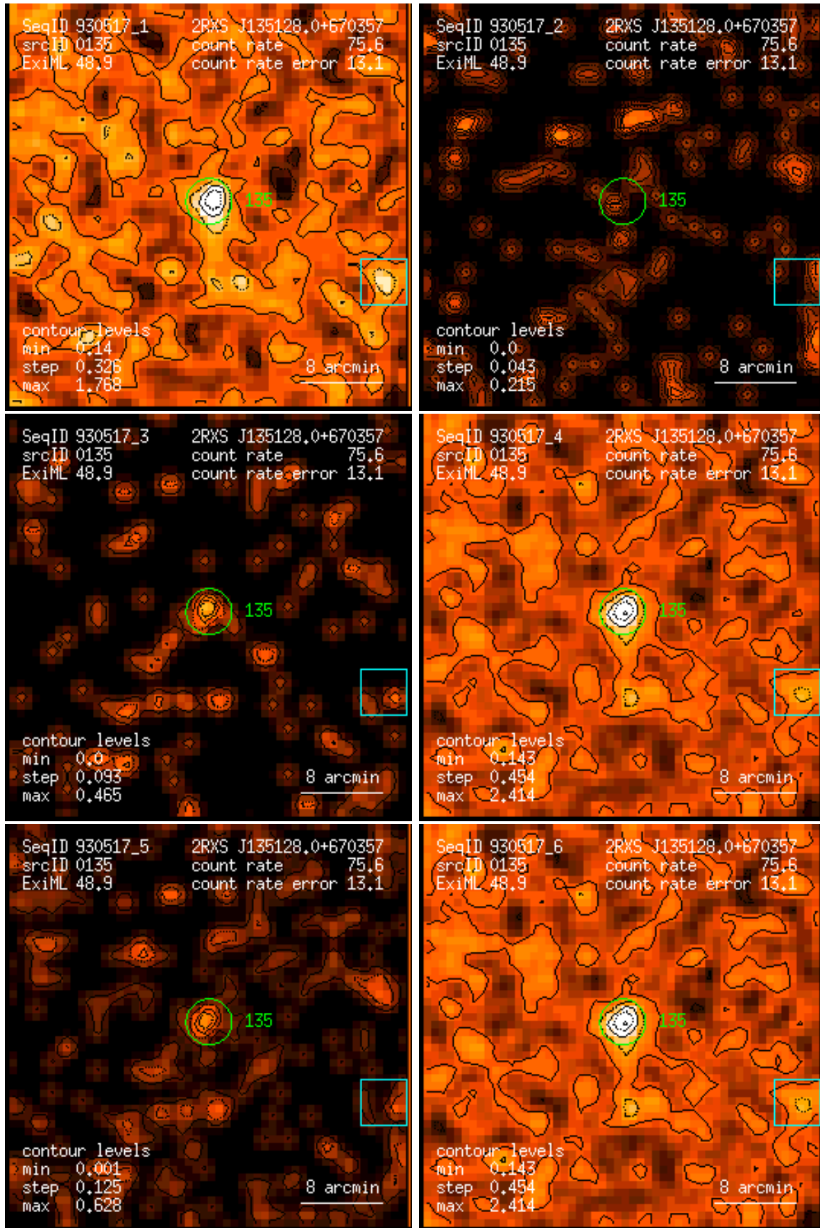
Figure 135: RASS 930517: detection 0135: band rate images, Gaussian filter: (1) PSPC channels 11 – 41, (2) 52 – 90, (3) 91 – 201, (4) 11 – 235, (5) 52 – 201, (6) 11 – 201. Broad band rates in counts/ks. Band rate contour levels in counts/ks/arcmin 2 .
