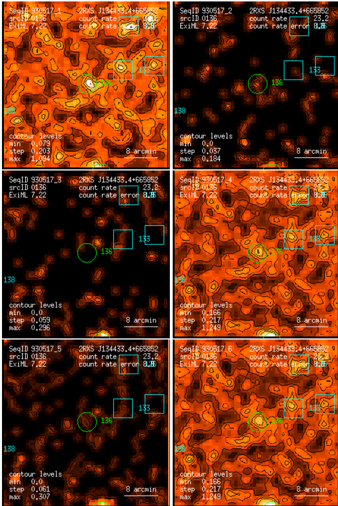
Figure 136: RASS 930517: detection 0136: band rate images, Gaussian filter: (1) PSPC channels 11 – 41, (2) 52 – 90, (3) 91 – 201, (4) 11 – 235, (5) 52 – 201, (6) 11 – 201. Broad band rates in counts/ks. Band rate contour levels in counts/ks/arcmin 2 .
