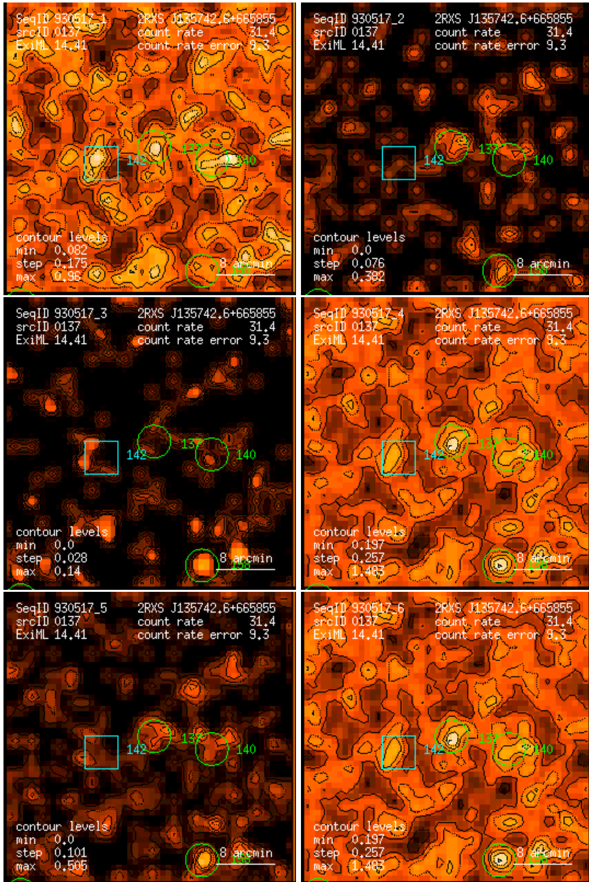
Figure 137: RASS 930517: detection 0137: band rate images, Gaussian filter: (1) PSPC channels 11 – 41, (2) 52 – 90, (3) 91 – 201, (4) 11 – 235, (5) 52 – 201, (6) 11 – 201. Broad band rates in counts/ks. Band rate contour levels in counts/ks/arcmin 2 .
