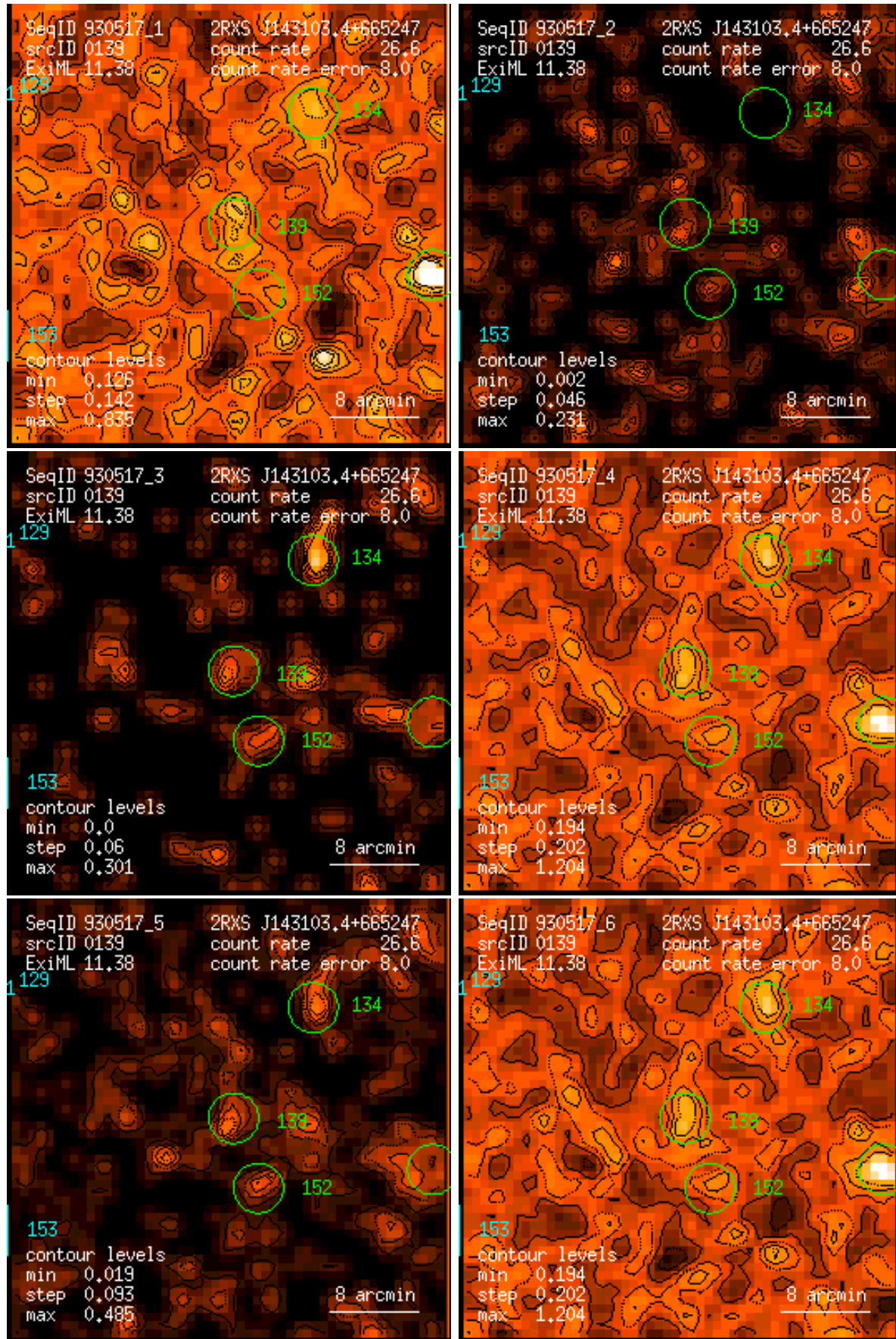
Figure 139: RASS 930517: detection 0139: band rate images, Gaussian filter: (1) PSPC channels 11 – 41, (2) 52 – 90, (3) 91 – 201, (4) 11 – 235, (5) 52 – 201, (6) 11 – 201. Broad band rates in counts/ks. Band rate contour levels in counts/ks/arcmin 2 .
