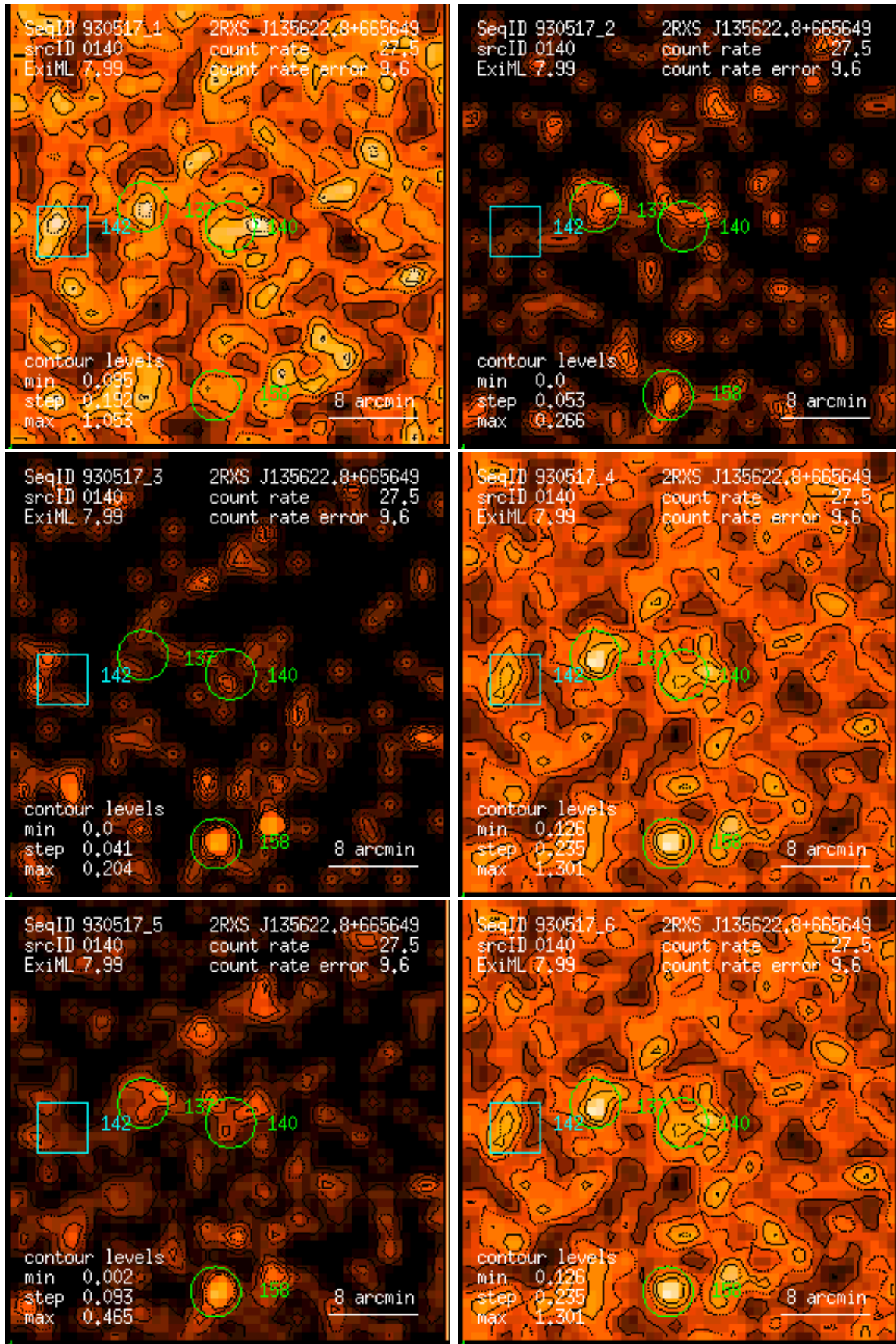
Figure 140: RASS 930517: detection 0140: band rate images, Gaussian filter: (1) PSPC channels 11 – 41, (2) 52 – 90, (3) 91 – 201, (4) 11 – 235, (5) 52 – 201, (6) 11 – 201. Broad band rates in counts/ks. Band rate contour levels in counts/ks/arcmin 2 .
