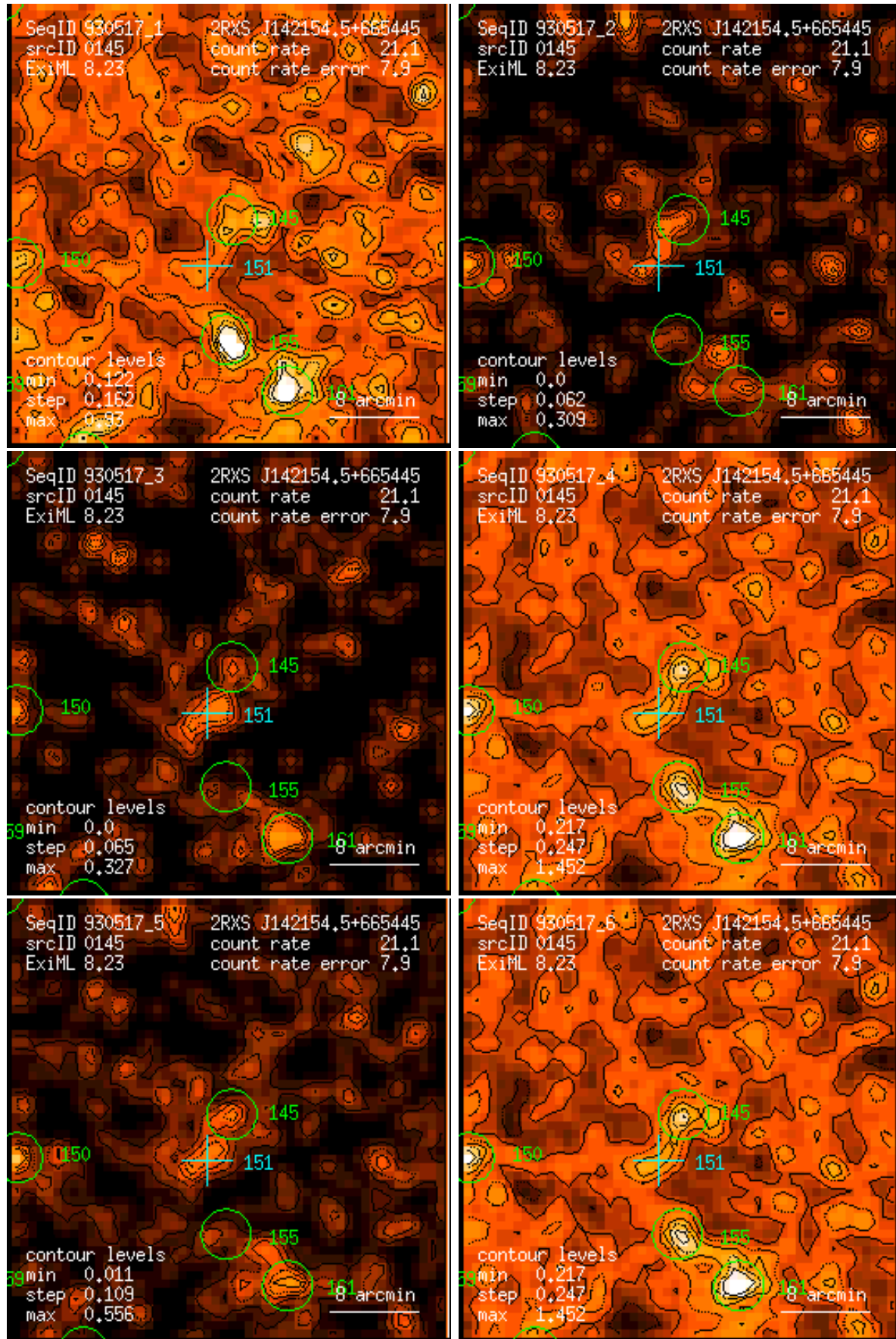
Figure 145: RASS 930517: detection 0145: band rate images, Gaussian filter: (1) PSPC channels 11 – 41, (2) 52 – 90, (3) 91 – 201, (4) 11 – 235, (5) 52 – 201, (6) 11 – 201. Broad band rates in counts/ks. Band rate contour levels in counts/ks/arcmin 2 .
