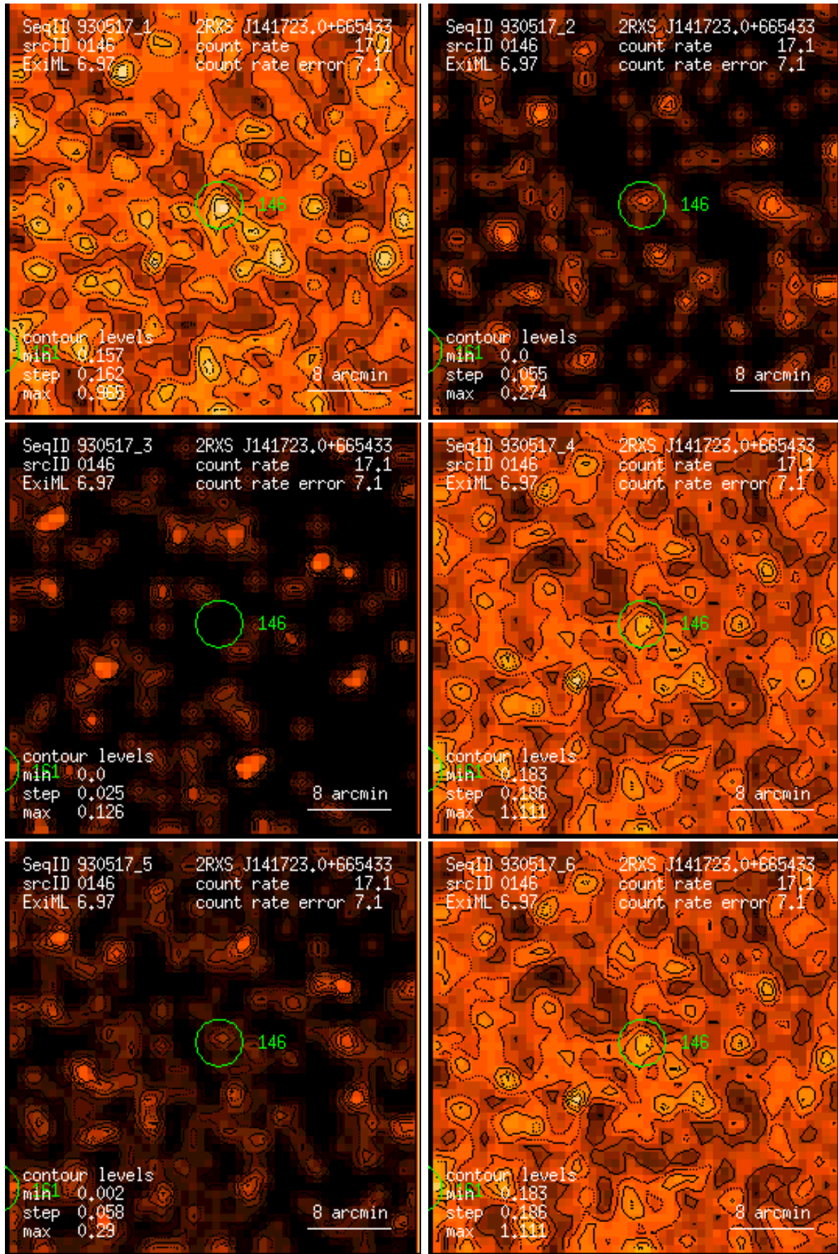
Figure 146: RASS 930517: detection 0146: band rate images, Gaussian filter: (1) PSPC channels 11 – 41, (2) 52 – 90, (3) 91 – 201, (4) 11 – 235, (5) 52 – 201, (6) 11 – 201. Broad band rates in counts/ks. Band rate contour levels in counts/ks/arcmin 2 .
