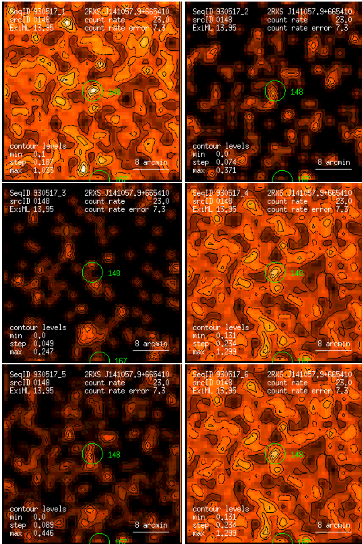
Figure 148: RASS 930517: detection 0148: band rate images, Gaussian filter: (1) PSPC channels 11 – 41, (2) 52 – 90, (3) 91 – 201, (4) 11 – 235, (5) 52 – 201, (6) 11 – 201. Broad band rates in counts/ks. Band rate contour levels in counts/ks/arcmin 2 .
