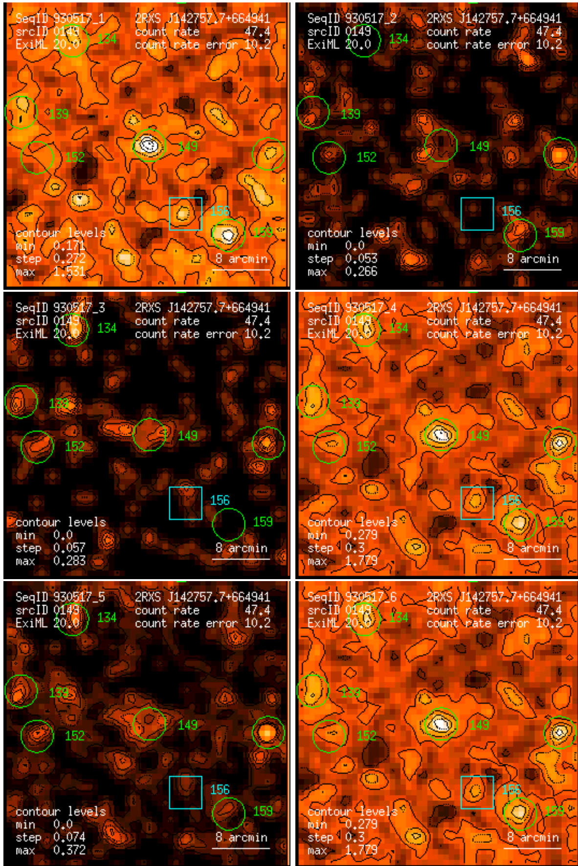
Figure 149: RASS 930517: detection 0149: band rate images, Gaussian filter: (1) PSPC channels 11 – 41, (2) 52 – 90, (3) 91 – 201, (4) 11 – 235, (5) 52 – 201, (6) 11 – 201. Broad band rates in counts/ks. Band rate contour levels in counts/ks/arcmin 2 .
