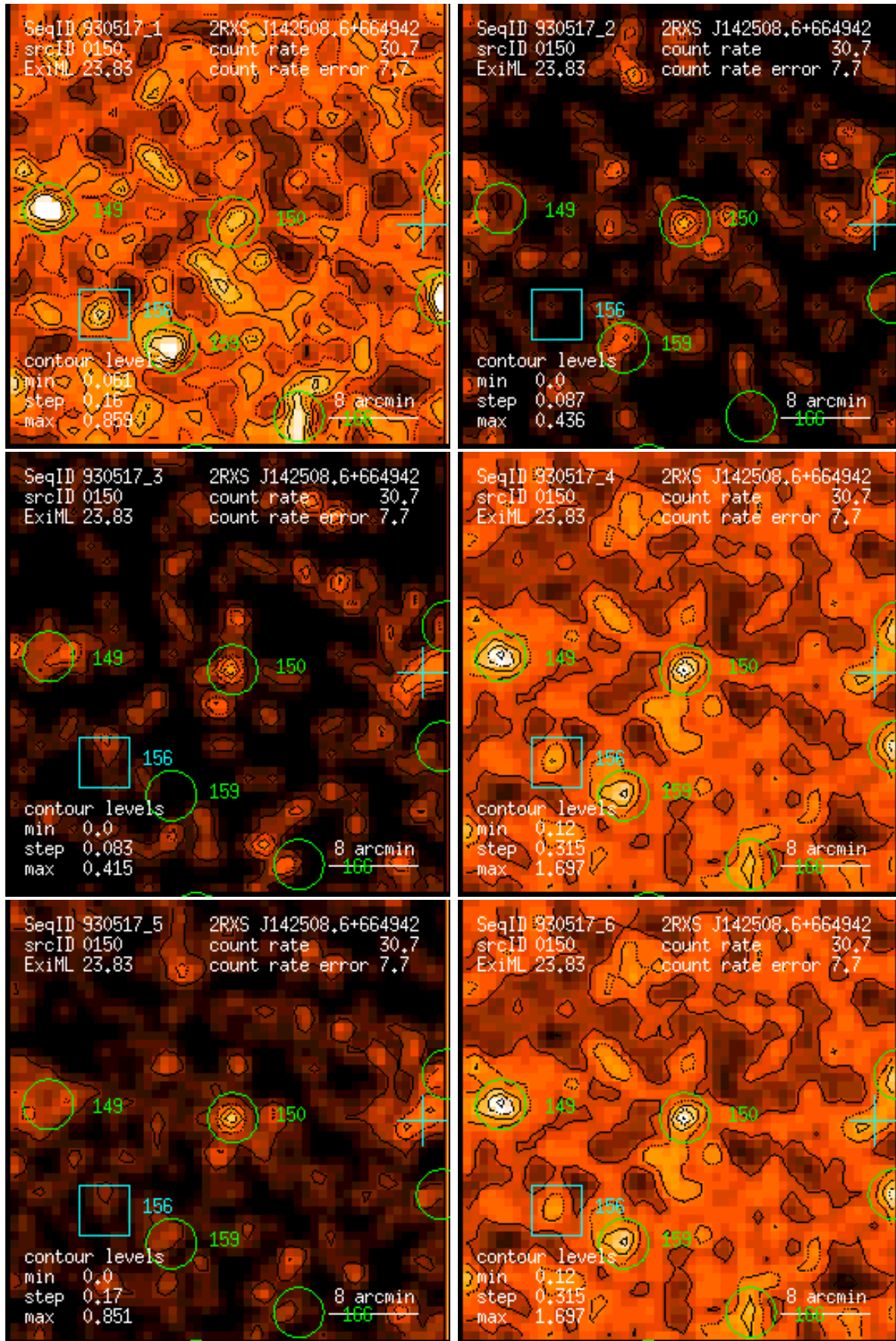
Figure 150: RASS 930517: detection 0150: band rate images, Gaussian filter: (1) PSPC channels 11 – 41, (2) 52 – 90, (3) 91 – 201, (4) 11 – 235, (5) 52 – 201, (6) 11 – 201. Broad band rates in counts/ks. Band rate contour levels in counts/ks/arcmin 2 .
