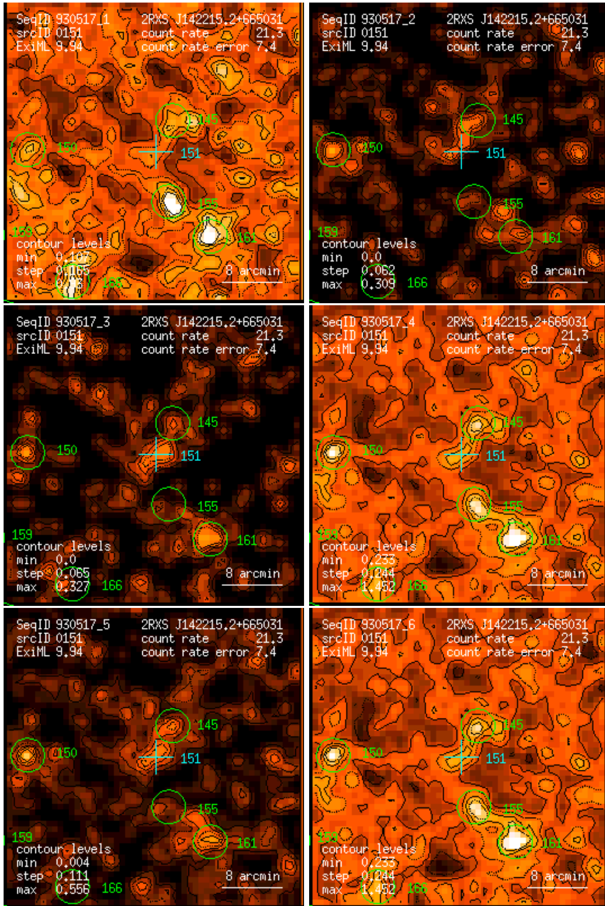
Figure 151: RASS 930517: detection 0151: band rate images, Gaussian filter: (1) PSPC channels 11 – 41, (2) 52 – 90, (3) 91 – 201, (4) 11 – 235, (5) 52 – 201, (6) 11 – 201. Broad band rates in counts/ks. Band rate contour levels in counts/ks/arcmin 2 .
