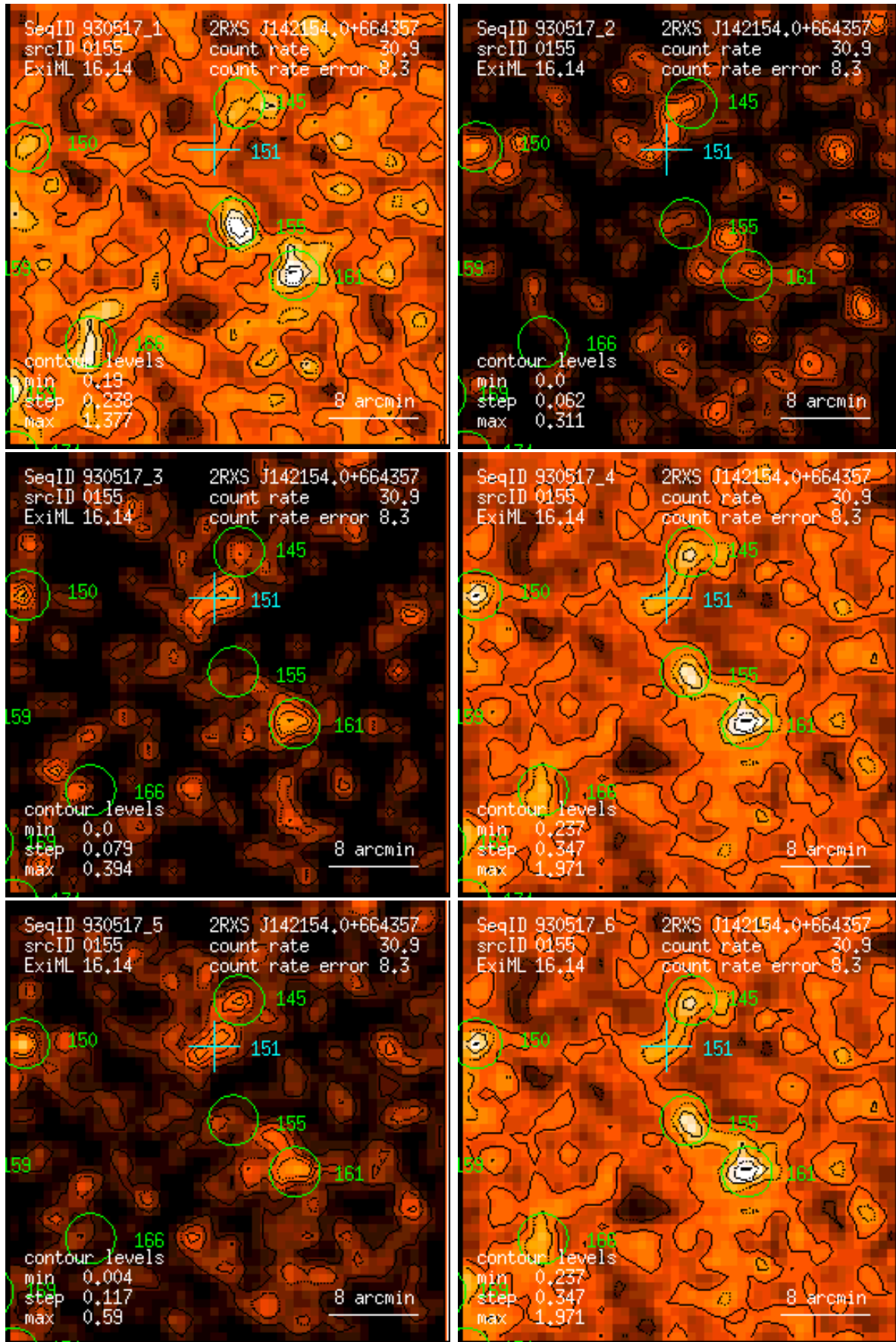
Figure 155: RASS 930517: detection 0155: band rate images, Gaussian filter: (1) PSPC channels 11 – 41, (2) 52 – 90, (3) 91 – 201, (4) 11 – 235, (5) 52 – 201, (6) 11 – 201. Broad band rates in counts/ks. Band rate contour levels in counts/ks/arcmin 2 .
