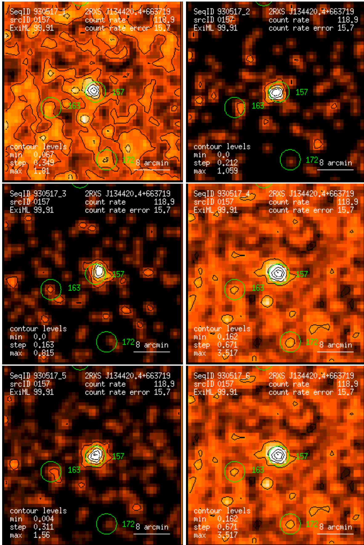
Figure 157: RASS 930517: detection 0157: band rate images, Gaussian filter: (1) PSPC channels 11 – 41, (2) 52 – 90, (3) 91 – 201, (4) 11 – 235, (5) 52 – 201, (6) 11 – 201. Broad band rates in counts/ks. Band rate contour levels in counts/ks/arcmin 2 .
