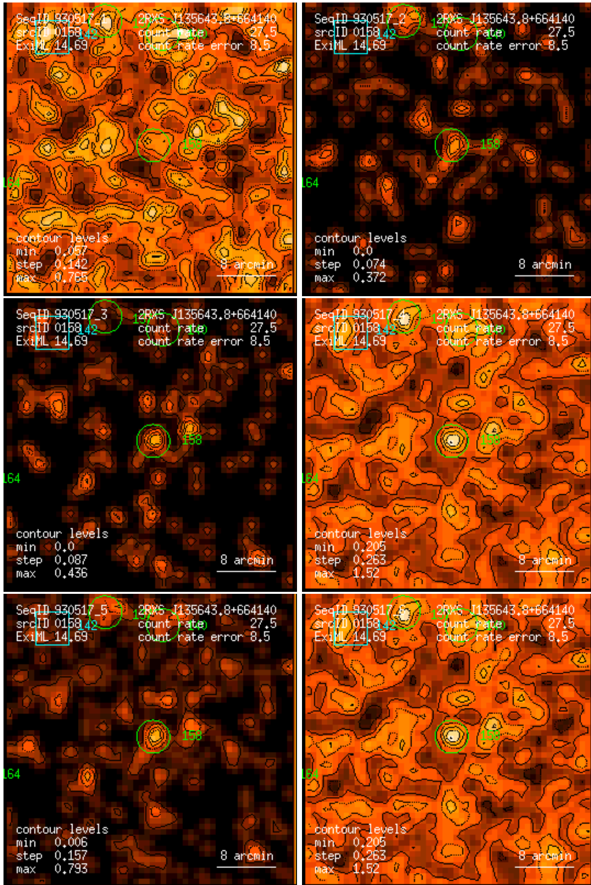
Figure 158: RASS 930517: detection 0158: band rate images, Gaussian filter: (1) PSPC channels 11 – 41, (2) 52 – 90, (3) 91 – 201, (4) 11 – 235, (5) 52 – 201, (6) 11 – 201. Broad band rates in counts/ks. Band rate contour levels in counts/ks/arcmin 2 .
