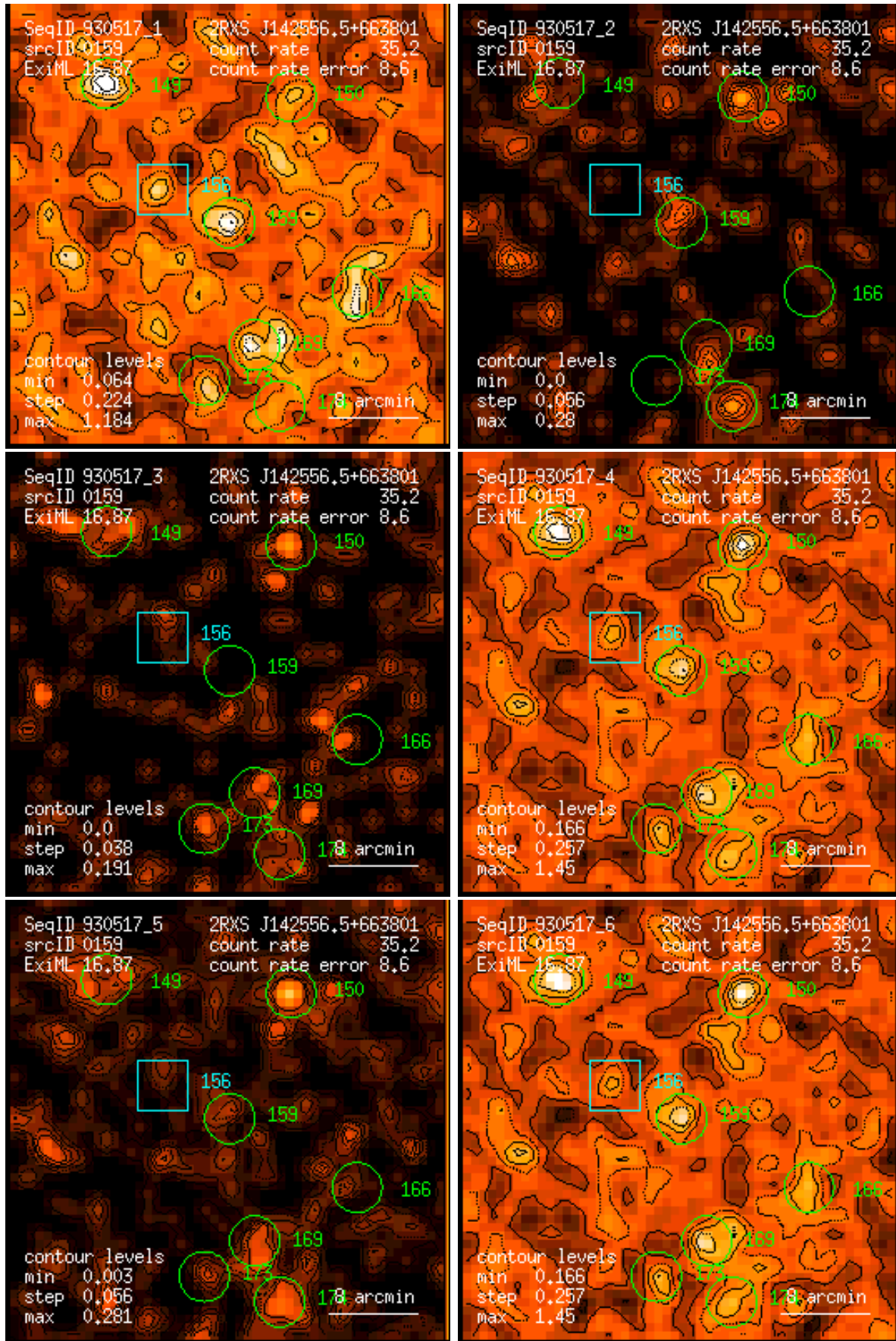
Figure 159: RASS 930517: detection 0159: band rate images, Gaussian filter: (1) PSPC channels 11 – 41, (2) 52 – 90, (3) 91 – 201, (4) 11 – 235, (5) 52 – 201, (6) 11 – 201. Broad band rates in counts/ks. Band rate contour levels in counts/ks/arcmin 2 .
