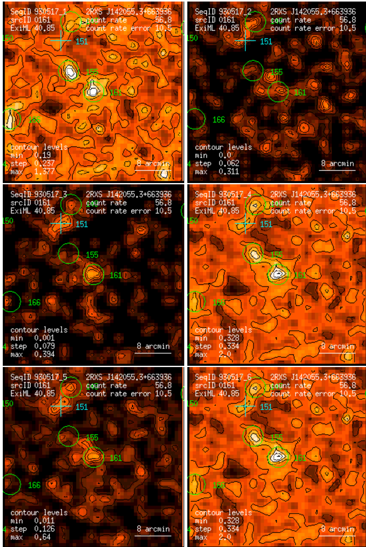
Figure 161: RASS 930517: detection 0161: band rate images, Gaussian filter: (1) PSPC channels 11 – 41, (2) 52 – 90, (3) 91 – 201, (4) 11 – 235, (5) 52 – 201, (6) 11 – 201. Broad band rates in counts/ks. Band rate contour levels in counts/ks/arcmin 2 .
