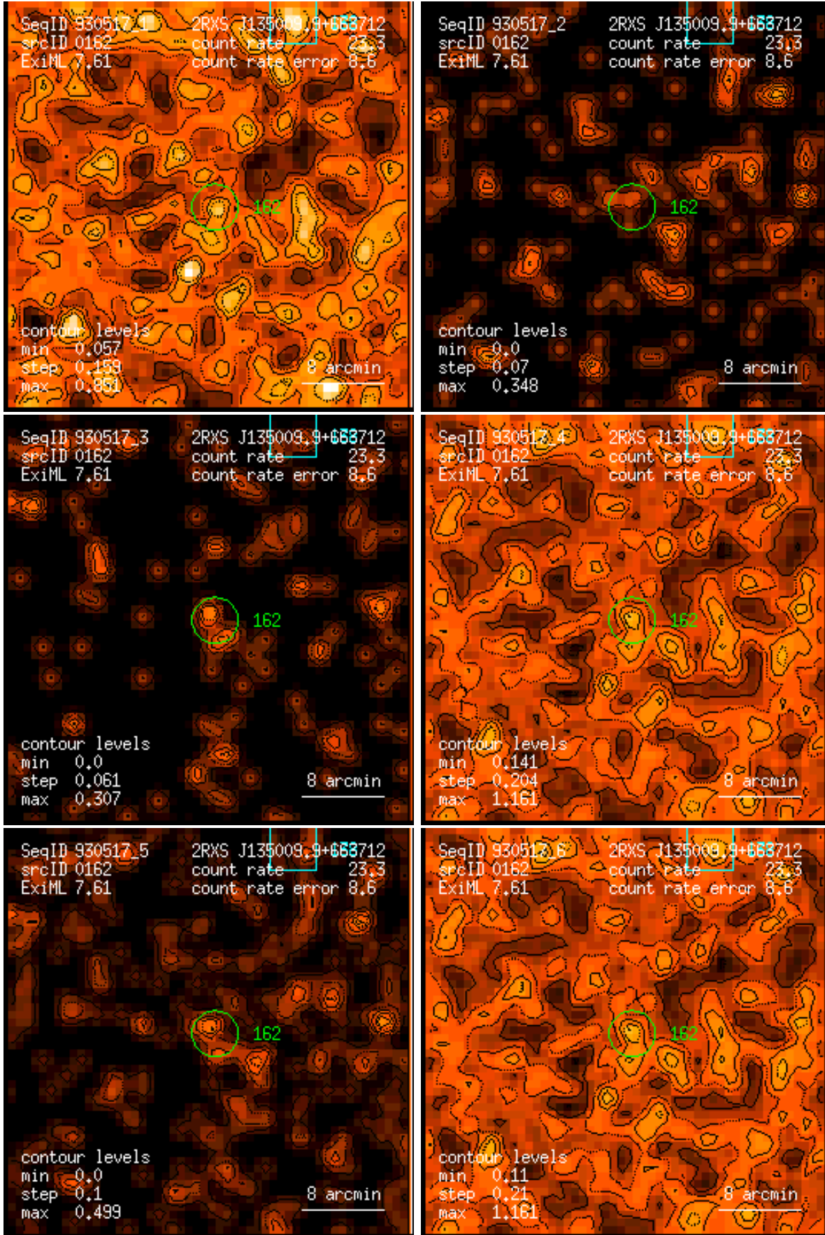
Figure 162: RASS 930517: detection 0162: band rate images, Gaussian filter: (1) PSPC channels 11 – 41, (2) 52 – 90, (3) 91 – 201, (4) 11 – 235, (5) 52 – 201, (6) 11 – 201. Broad band rates in counts/ks. Band rate contour levels in counts/ks/arcmin 2 .
