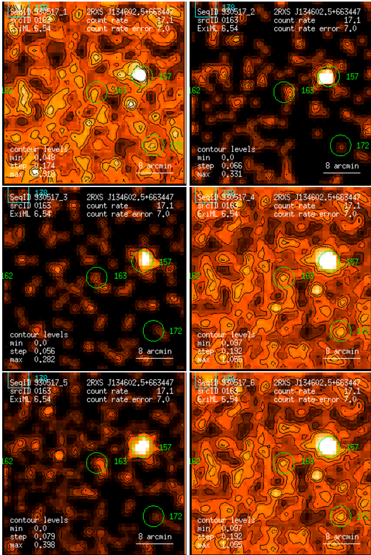
Figure 163: RASS 930517: detection 0163: band rate images, Gaussian filter: (1) PSPC channels 11 – 41, (2) 52 – 90, (3) 91 – 201, (4) 11 – 235, (5) 52 – 201, (6) 11 – 201. Broad band rates in counts/ks. Band rate contour levels in counts/ks/arcmin 2 .
