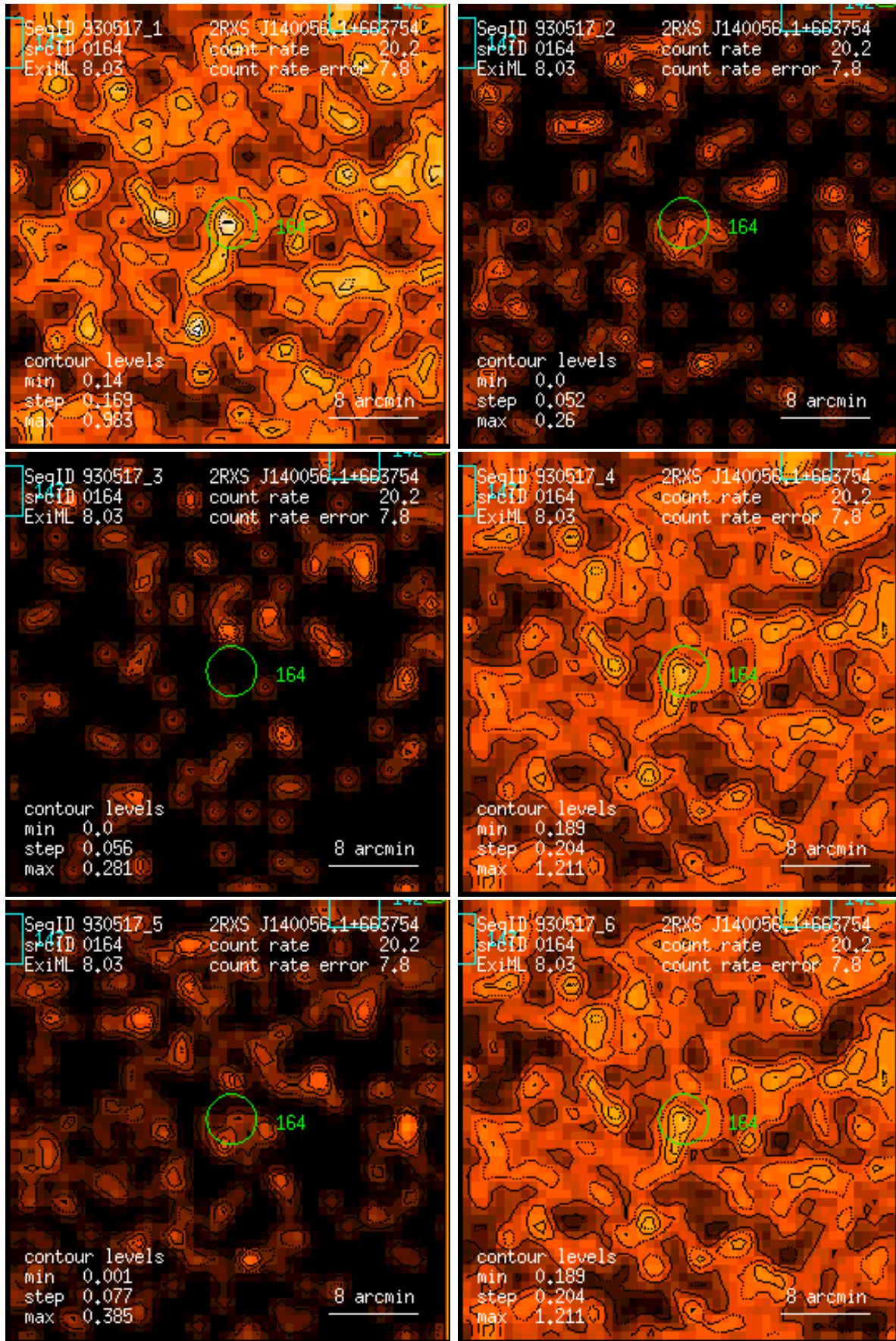
Figure 164: RASS 930517: detection 0164: band rate images, Gaussian filter: (1) PSPC channels 11 – 41, (2) 52 – 90, (3) 91 – 201, (4) 11 – 235, (5) 52 – 201, (6) 11 – 201. Broad band rates in counts/ks. Band rate contour levels in counts/ks/arcmin 2 .
