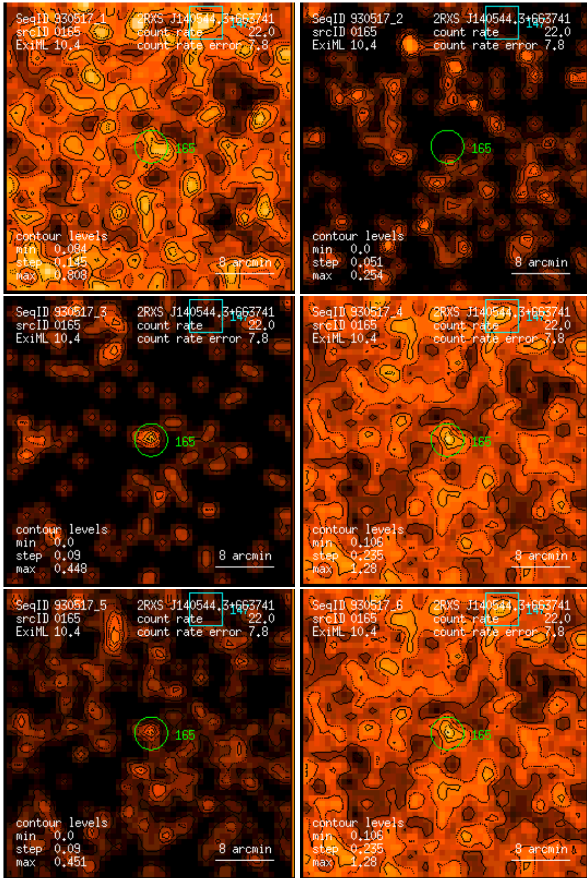
Figure 165: RASS 930517: detection 0165: band rate images, Gaussian filter: (1) PSPC channels 11 – 41, (2) 52 – 90, (3) 91 – 201, (4) 11 – 235, (5) 52 – 201, (6) 11 – 201. Broad band rates in counts/ks. Band rate contour levels in counts/ks/arcmin 2 .
