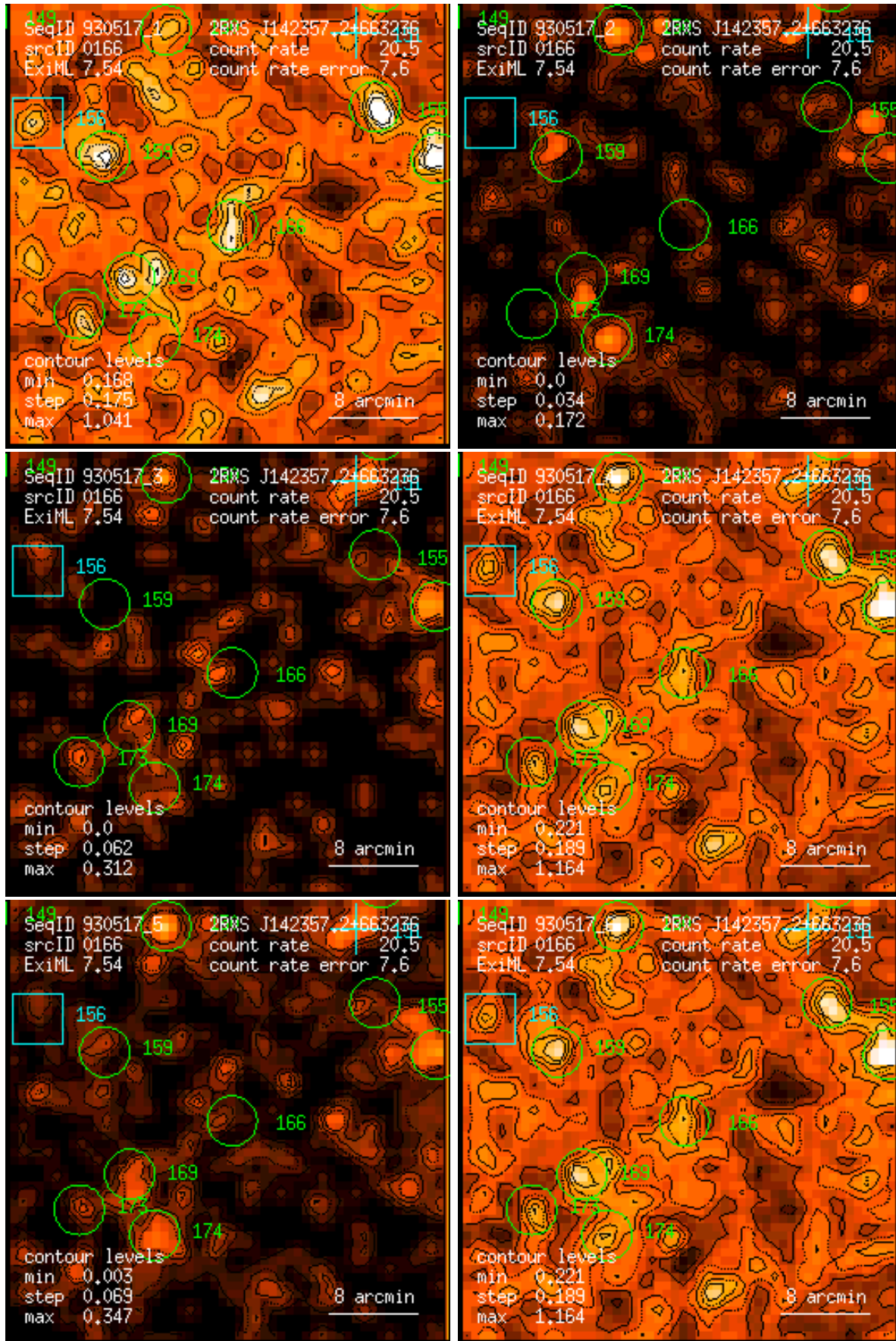
Figure 166: RASS 930517: detection 0166: band rate images, Gaussian filter: (1) PSPC channels 11 – 41, (2) 52 – 90, (3) 91 – 201, (4) 11 – 235, (5) 52 – 201, (6) 11 – 201. Broad band rates in counts/ks. Band rate contour levels in counts/ks/arcmin 2 .
