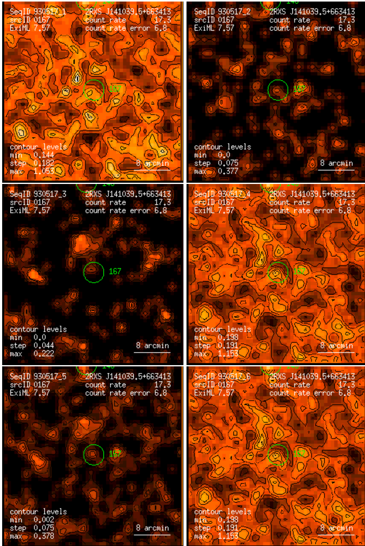
Figure 167: RASS 930517: detection 0167: band rate images, Gaussian filter: (1) PSPC channels 11 – 41, (2) 52 – 90, (3) 91 – 201, (4) 11 – 235, (5) 52 – 201, (6) 11 – 201. Broad band rates in counts/ks. Band rate contour levels in counts/ks/arcmin 2 .
