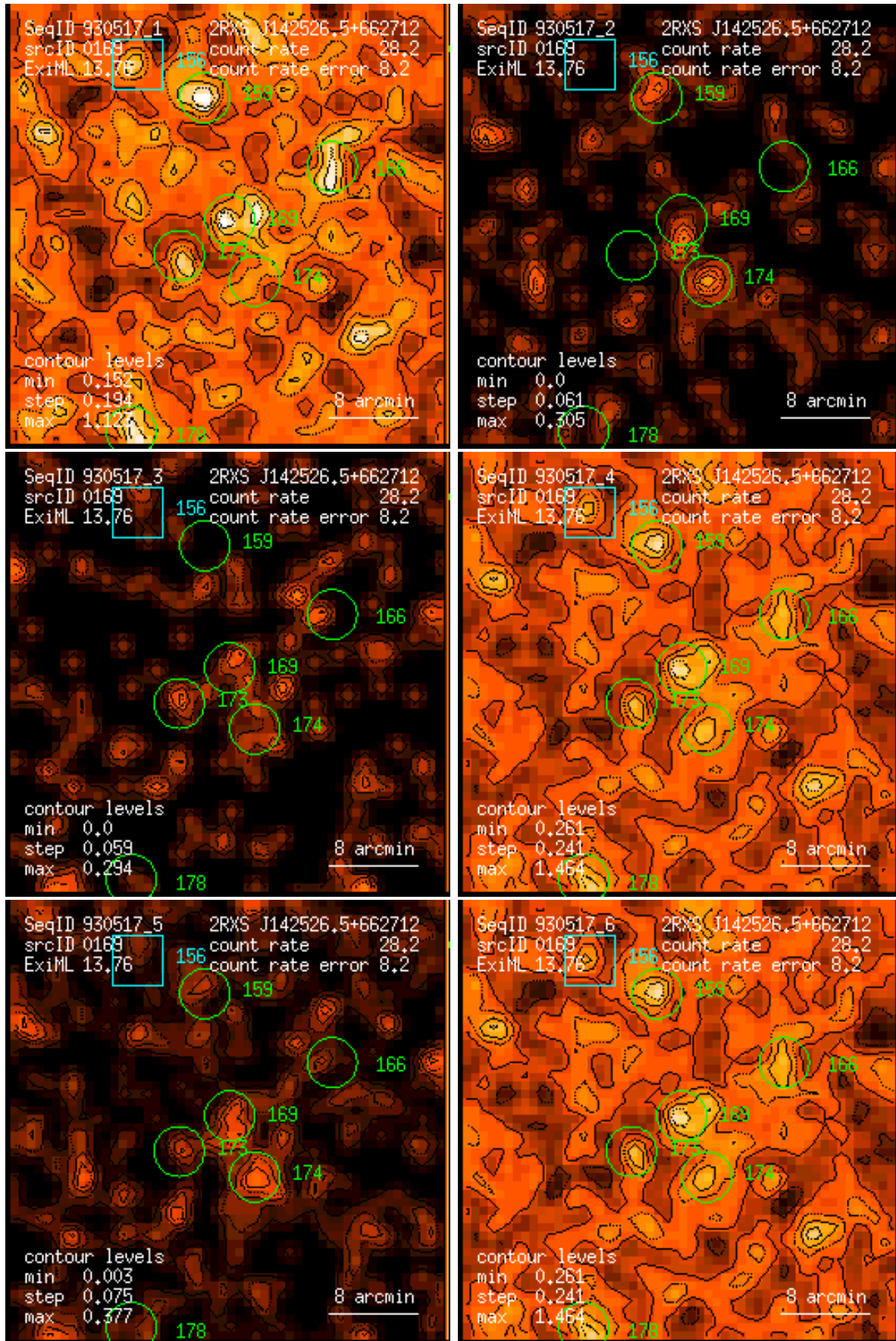
Figure 169: RASS 930517: detection 0169: band rate images, Gaussian filter: (1) PSPC channels 11 – 41, (2) 52 – 90, (3) 91 – 201, (4) 11 – 235, (5) 52 – 201, (6) 11 – 201. Broad band rates in counts/ks. Band rate contour levels in counts/ks/arcmin 2 .
