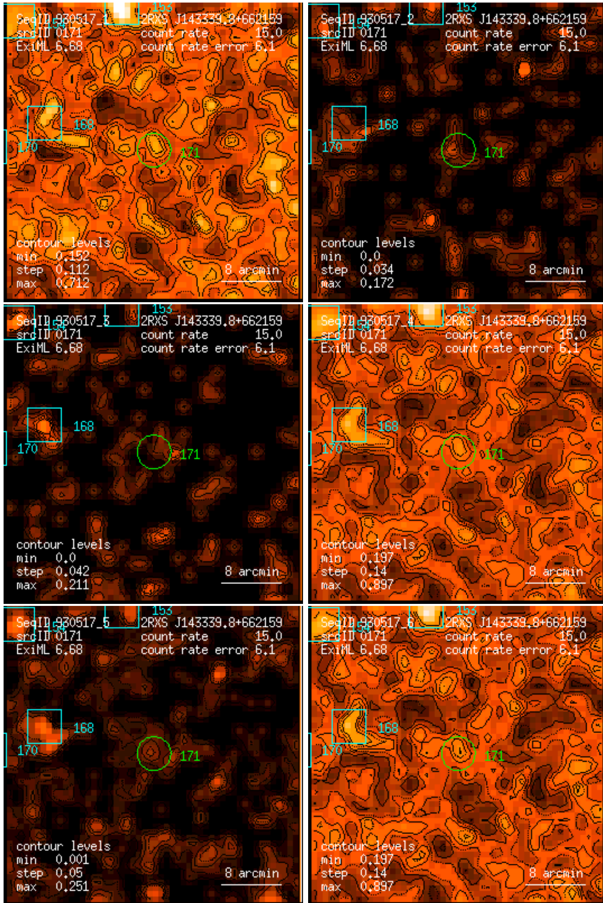
Figure 171: RASS 930517: detection 0171: band rate images, Gaussian filter: (1) PSPC channels 11 – 41, (2) 52 – 90, (3) 91 – 201, (4) 11 – 235, (5) 52 – 201, (6) 11 – 201. Broad band rates in counts/ks. Band rate contour levels in counts/ks/arcmin 2 .
