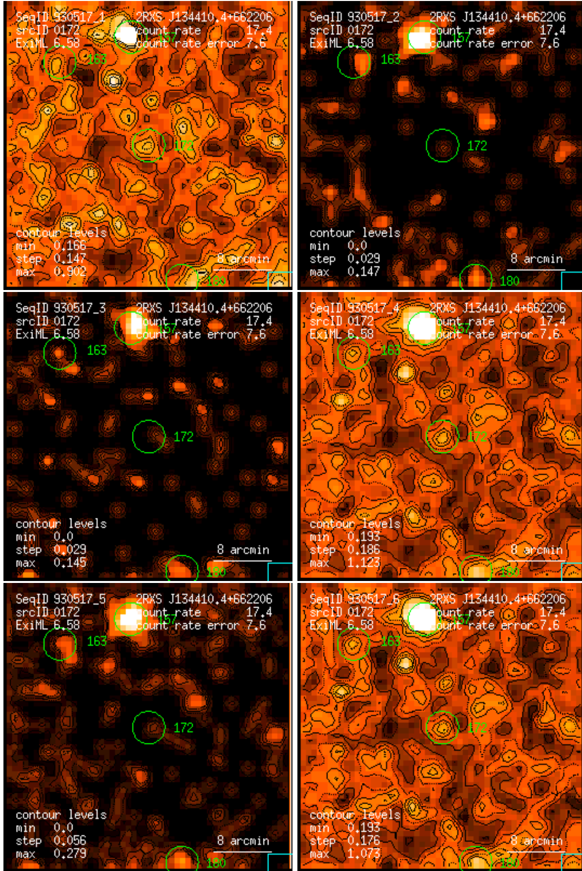
Figure 172: RASS 930517: detection 0172: band rate images, Gaussian filter: (1) PSPC channels 11 – 41, (2) 52 – 90, (3) 91 – 201, (4) 11 – 235, (5) 52 – 201, (6) 11 – 201. Broad band rates in counts/ks. Band rate contour levels in counts/ks/arcmin 2 .
