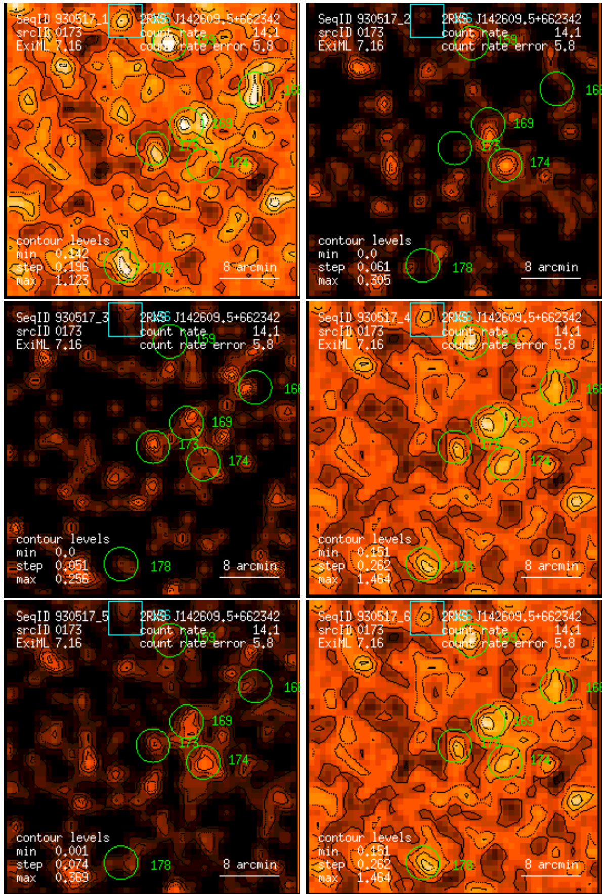
Figure 173: RASS 930517: detection 0173: band rate images, Gaussian filter: (1) PSPC channels 11 – 41, (2) 52 – 90, (3) 91 – 201, (4) 11 – 235, (5) 52 – 201, (6) 11 – 201. Broad band rates in counts/ks. Band rate contour levels in counts/ks/arcmin 2 .
