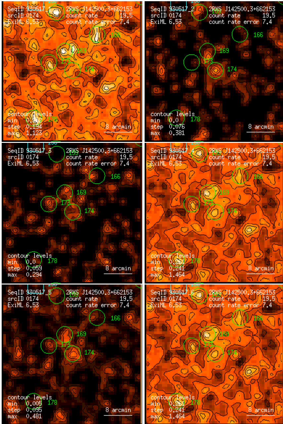
Figure 174: RASS 930517: detection 0174: band rate images, Gaussian filter: (1) PSPC channels 11 – 41, (2) 52 – 90, (3) 91 – 201, (4) 11 – 235, (5) 52 – 201, (6) 11 – 201. Broad band rates in counts/ks. Band rate contour levels in counts/ks/arcmin 2 .
