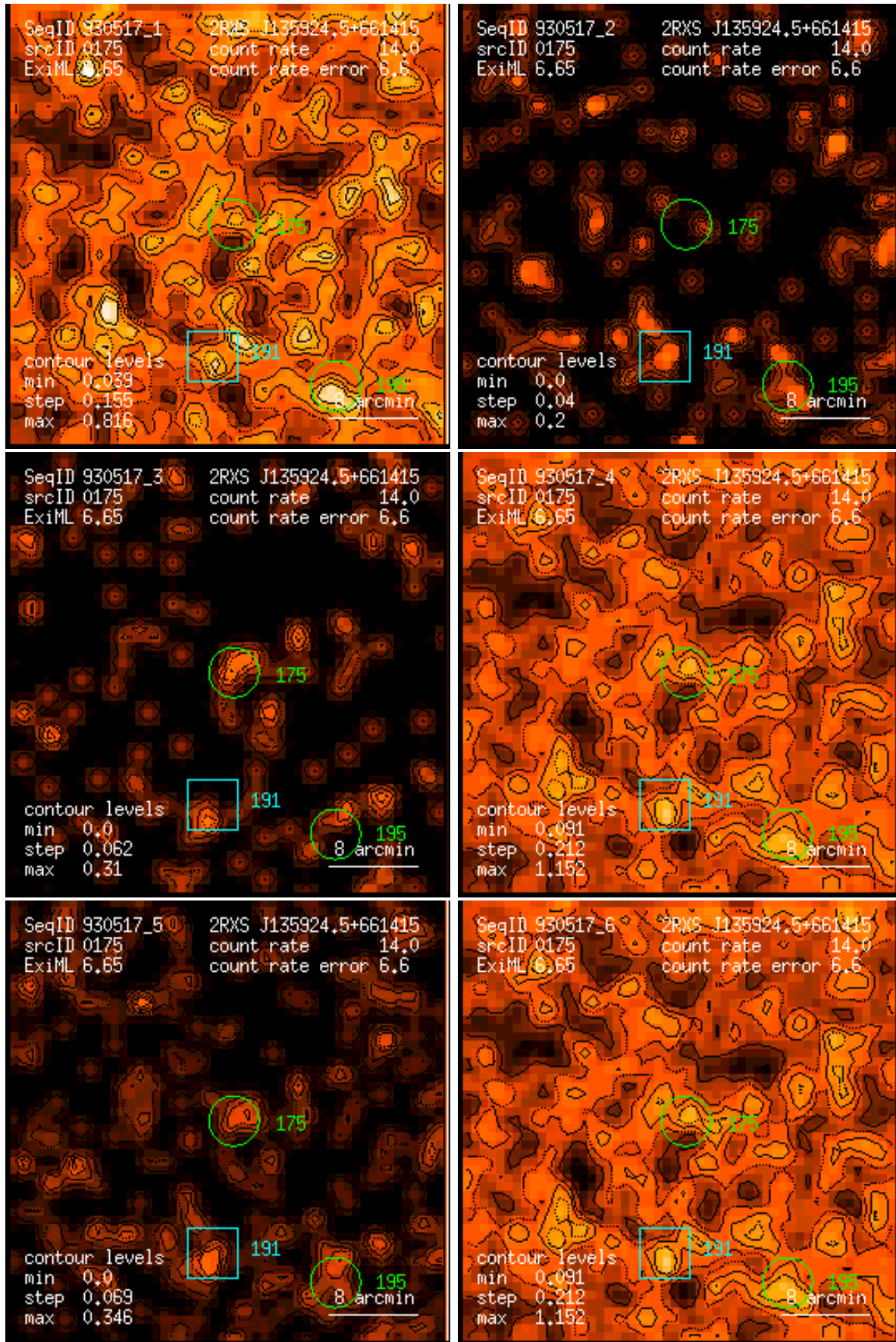
Figure 175: RASS 930517: detection 0175: band rate images, Gaussian filter: (1) PSPC channels 11 – 41, (2) 52 – 90, (3) 91 – 201, (4) 11 – 235, (5) 52 – 201, (6) 11 – 201. Broad band rates in counts/ks. Band rate contour levels in counts/ks/arcmin 2 .
