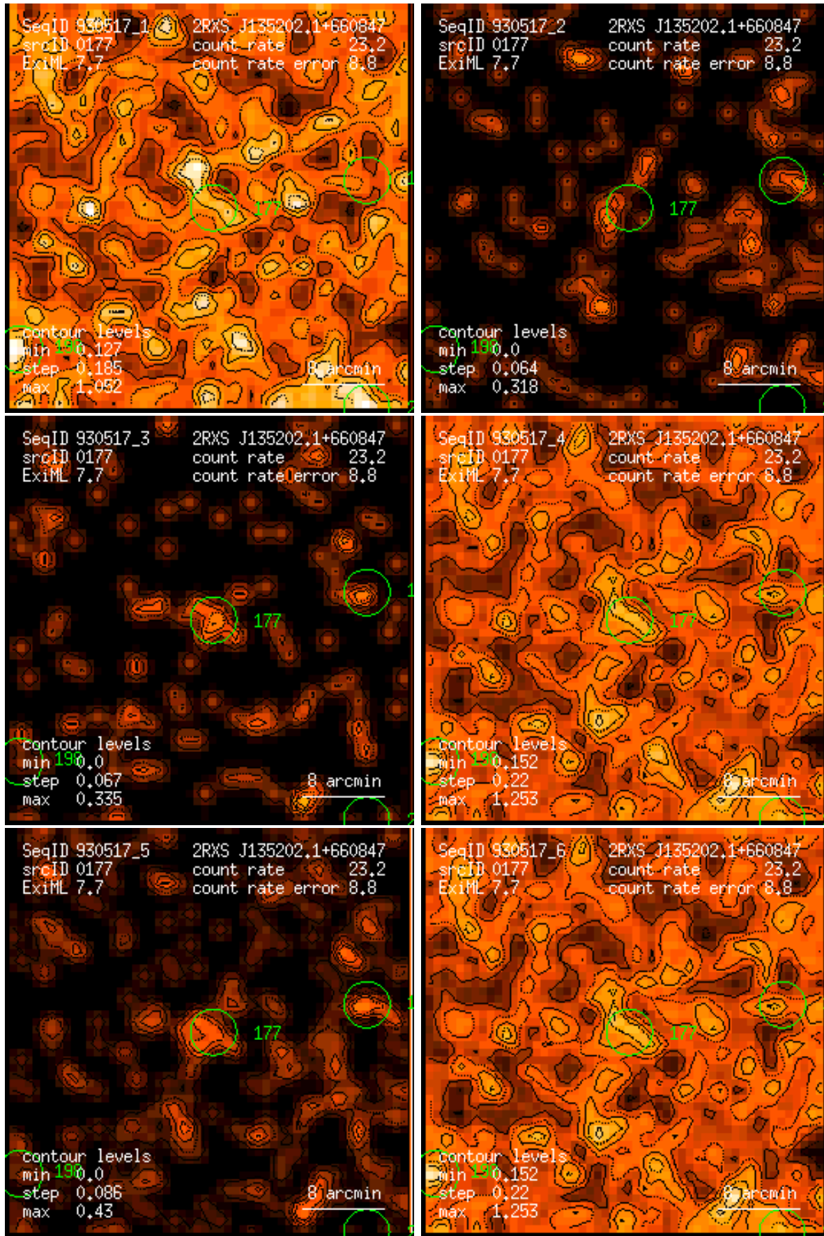
Figure 177: RASS 930517: detection 0177: band rate images, Gaussian filter: (1) PSPC channels 11 – 41, (2) 52 – 90, (3) 91 – 201, (4) 11 – 235, (5) 52 – 201, (6) 11 – 201. Broad band rates in counts/ks. Band rate contour levels in counts/ks/arcmin 2 .
