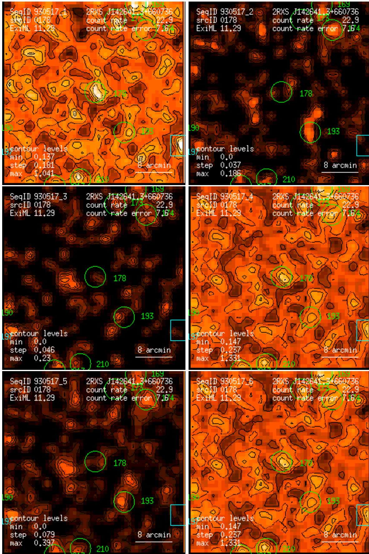
Figure 178: RASS 930517: detection 0178: band rate images, Gaussian filter: (1) PSPC channels 11 – 41, (2) 52 – 90, (3) 91 – 201, (4) 11 – 235, (5) 52 – 201, (6) 11 – 201. Broad band rates in counts/ks. Band rate contour levels in counts/ks/arcmin 2 .
