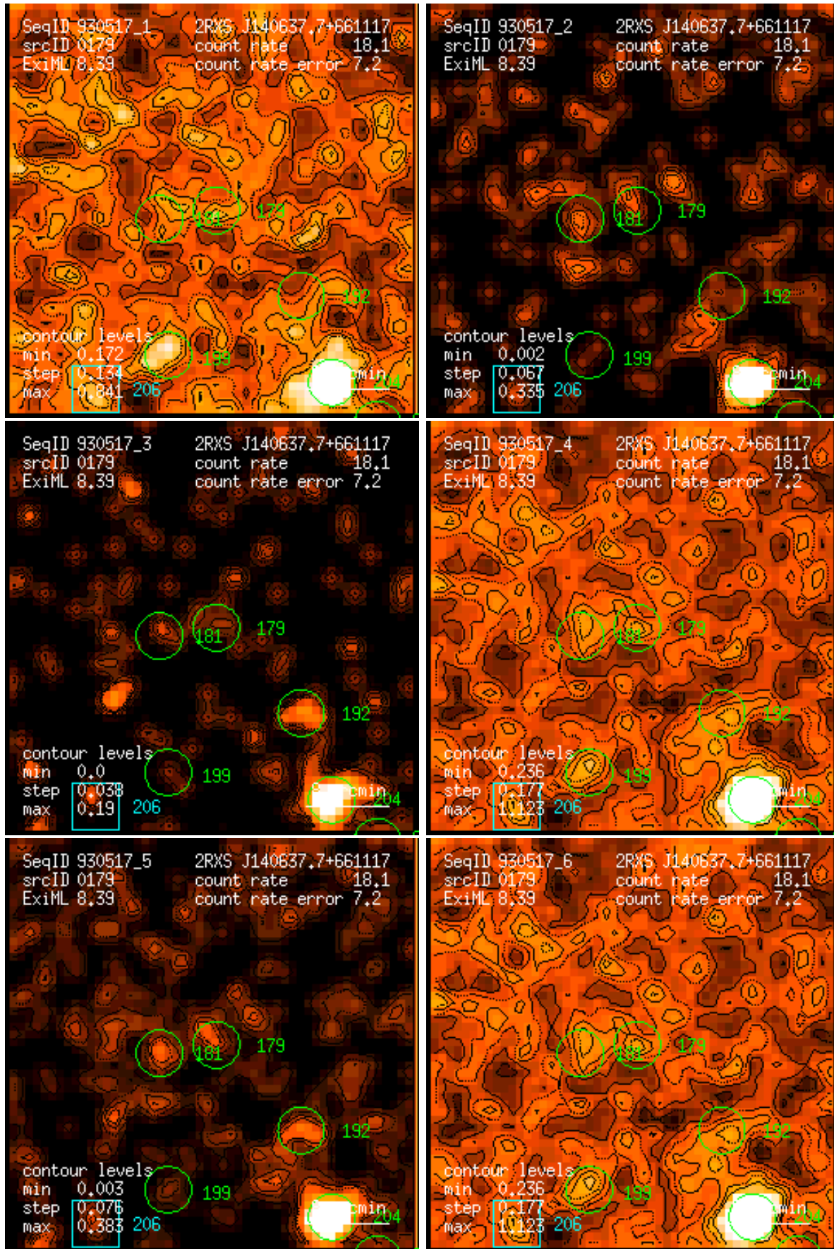
Figure 179: RASS 930517: detection 0179: band rate images, Gaussian filter: (1) PSPC channels 11 – 41, (2) 52 – 90, (3) 91 – 201, (4) 11 – 235, (5) 52 – 201, (6) 11 – 201. Broad band rates in counts/ks. Band rate contour levels in counts/ks/arcmin 2 .
