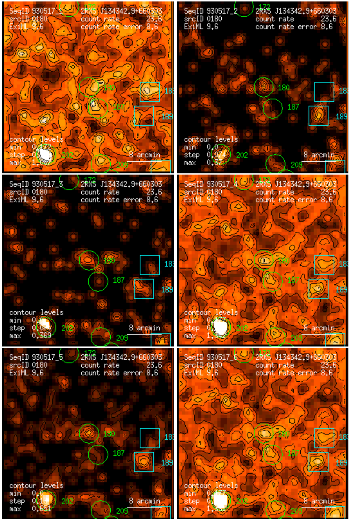
Figure 180: RASS 930517: detection 0180: band rate images, Gaussian filter: (1) PSPC channels 11 – 41, (2) 52 – 90, (3) 91 – 201, (4) 11 – 235, (5) 52 – 201, (6) 11 – 201. Broad band rates in counts/ks. Band rate contour levels in counts/ks/arcmin 2 .
