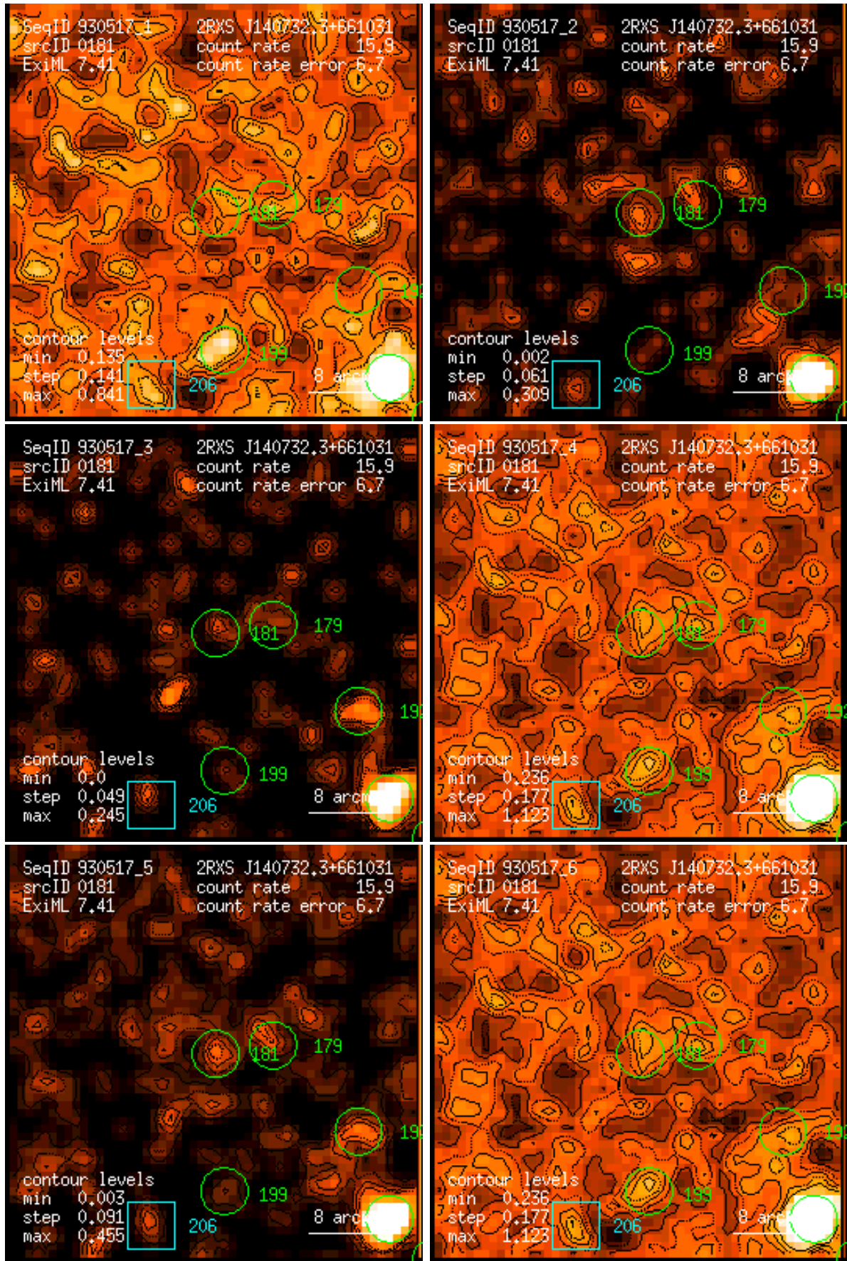
Figure 181: RASS 930517: detection 0181: band rate images, Gaussian filter: (1) PSPC channels 11 – 41, (2) 52 – 90, (3) 91 – 201, (4) 11 – 235, (5) 52 – 201, (6) 11 – 201. Broad band rates in counts/ks. Band rate contour levels in counts/ks/arcmin 2 .
